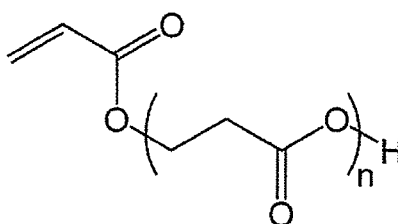
beta-carboxyethyl acrylate
