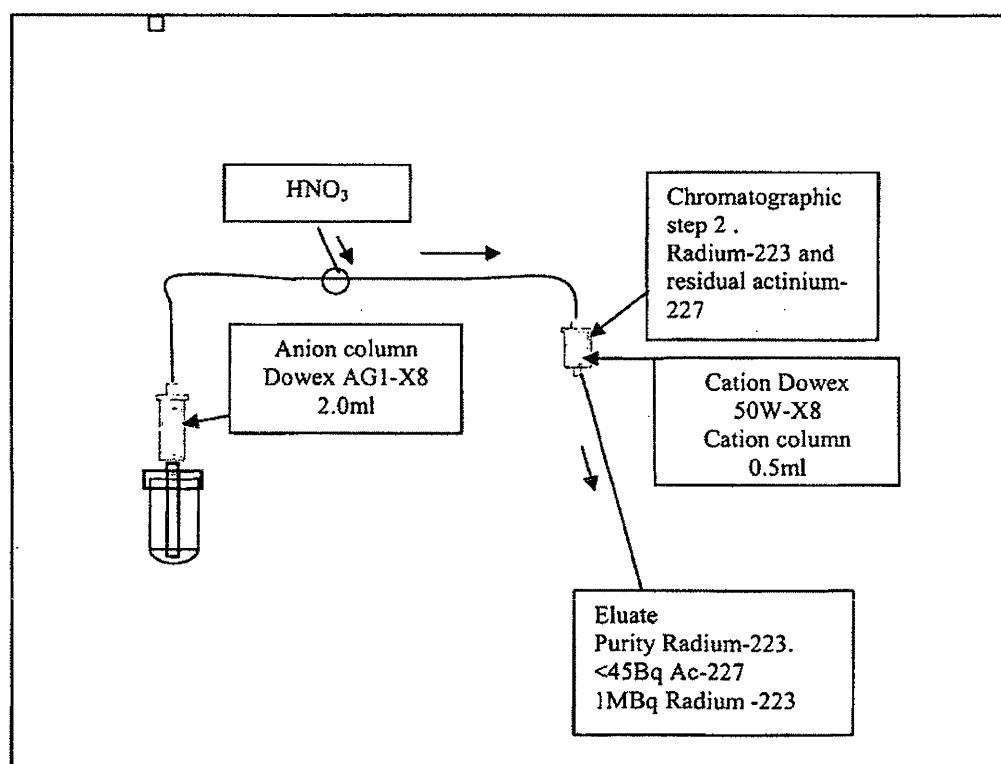
Figure 4 - setup for evaluating cation separation column.
