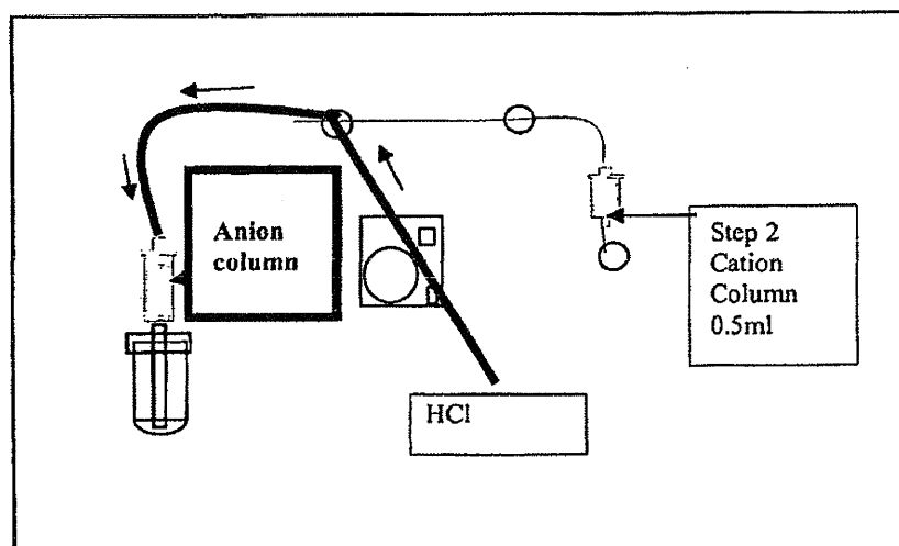
Figure 8 - regeneration of parent isotopes after radium separation.
