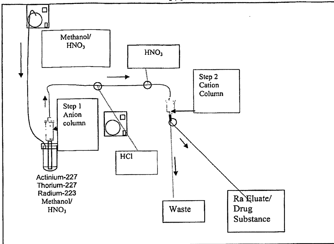
Figure 9 - Full scale experimental setup
