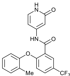
N-(2-oxo-1,2-dihydropyridin-4-yl)-2-(o-tolyloxy)-5-(trifluoromethyl)benzamide;
