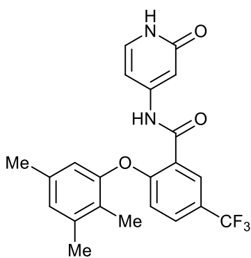
N-(2-oxo-1,2-dihydropyridin-4-yl)-5-(trifluoromethyl)-2-(2,3,5-trimethylphenoxy)benzamide;
