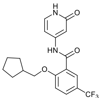
2-(cyclopentylmethoxy)-N-(2-oxo-1,2-dihydropyridin-4-yl)-5-(trifluoromethyl)benzamide;
