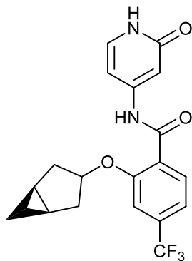
2-((1R,5S)-bicyclo[3.1.0]hexan-3-yloxy)-N-(2-oxo-1,2-dihydropyridin-4-yl)-4-(trifluoromethyl)benzamide;
