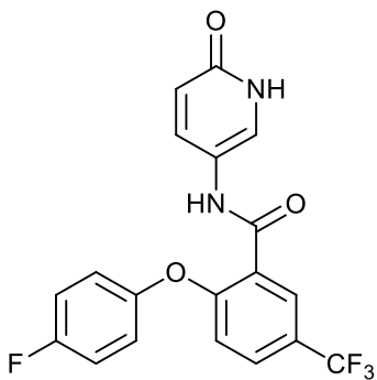
2-(4-fluorophenoxy)-N-(6-oxo-1,6-dihydropyridin-3-yl)-5-(trifluoromethyl)benzamide;
