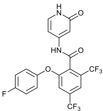
2-(4-fluorophenoxy)-N-(2-oxo-1,2-dihydropyridin-4-yl)-4,6-bis(trifluoromethyl)benzamide;
