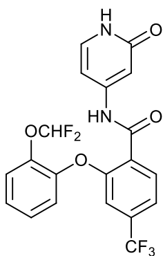
2-(2-(difluoromethoxy)phenoxy)-N-(2-oxo-1,2-dihydropyridin-4-yl)-4-(trifluoromethyl)benzamide;
