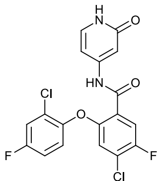
4-chloro-2-(2-chloro-4-fluorophenoxy)-5-fluoro-N-(2-oxo-1,2-dihydropyridin-4-yl)benzamide;
