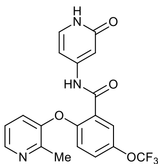
2-((2-methylpyridin-3-yl)oxy)-N-(2-oxo-1,2-dihydropyridin-4-yl)-5-(trifluoromethoxy)benzamide;
