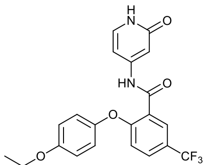
2-(4-ethoxyphenoxy)-N-(2-oxo-1,2-dihydropyridin-4-yl)-5-(trifluoromethyl)benzamide;
