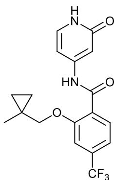
2-((1-methylcyclopropyl)methoxy)-N-(2-oxo-1,2-dihydropyridin-4-yl)-4-(trifluoromethyl)benzamide;
