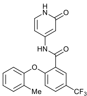
N-(2-oxo-1,2-dihydropyridin-4-yl)-2-(o-tolylloxy)-5-(trifluoromethyl)benzamide;
