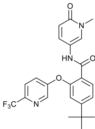
4-(tert-butyl)-N-(1-methyl-6-oxo-1,6-dihydropyridin-3-yl)-2-((6-(trifluoromethyl)pyridin-3-yl)oxy)benzamide;
