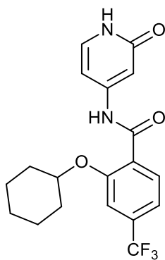
2-(cyclohexyloxy)-N-(2-oxo-1,2-dihydropyridin-4-yl)-4-(trifluoromethyl)benzamide;
