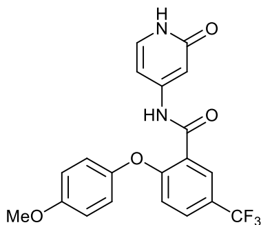
2-(4-methoxyphenoxy)-N-(2-oxo-1,2-dihydropyridin-4-yl)-5-(trifluoromethyl)benzamide;
