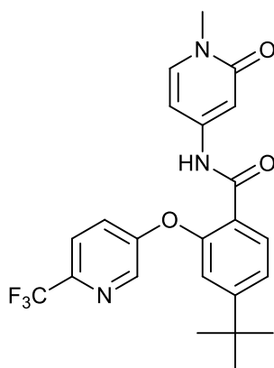
4-(tert-butyl)-N-(1-methyl-2-oxo-1,2-dihydropyridin-4-yl)-2-((6-(trifluoromethyl)pyridin-3-yl)oxy)benzamide;
