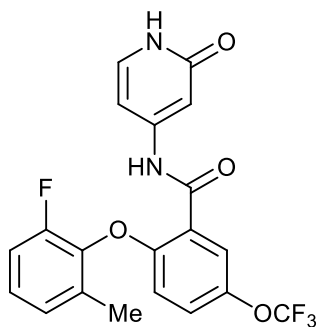
2-(2-fluoro-6-methylphenoxy)-N-(2-oxo-1,2-dihydropyridin-4-yl)-5-(trifluoromethoxy)benzamide;
