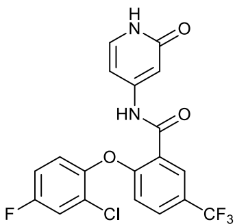
2-(2-chloro-4-fluorophenoxy)-N-(2-oxo-1,2-dihydropyridin-4-yl)-5-(trifluoromethyl)benzamide;
