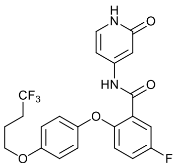
5-fluoro-N-(2-oxo-1,2-dihydropyridin-4-yl)-2-(4-(4,4,4-trifluorobutoxy)phenoxy)benzamide.
