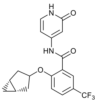
2-((1R,5S)-bicyclo[3.1.0]hexan-3-yloxy)-N-(2-oxo-1,2-dihydropyridin-4-yl)-5-(trifluoromethyl)benzamide;
