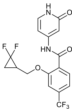
2-((2,2-difluorocyclopropyl)methoxy)-N-(2-oxo-1,2-dihydropyridin-4-yl)-4-(trifluoromethyl)benzamide;
