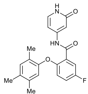
5-fluoro-N-(2-oxo-1,2-dihydropyridin-4-yl)-2-(2,4,5-trimethylphenoxy)benzamide;
