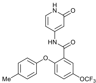
N-(2-oxo-1,2-dihydropyridin-4-yl)-2-(p-tolyloxy)-5-(trifluoromethoxy)benzamide;
