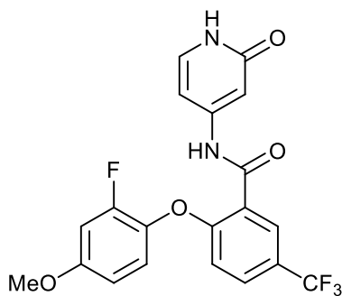
2-(2-fluoro-4-methoxyphenoxy)-N-(2-oxo-1,2-dihydropyridin-4-yl)-5-(trifluoromethyl)benzamide;
