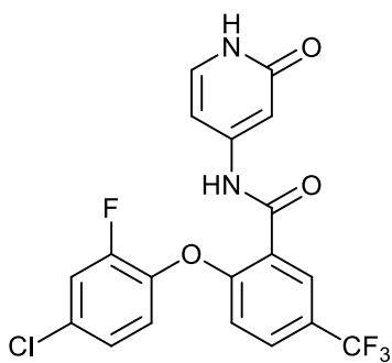
2-(4-chloro-2-fluorophenoxy)-N-(2-oxo-1,2-dihydropyridin-4-yl)-5-(trifluoromethyl)benzamide;
