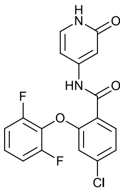
4-chloro-2-(2,6-difluorophenoxy)-N-(2-oxo-1,2-dihydropyridin-4-yl)benzamide;
