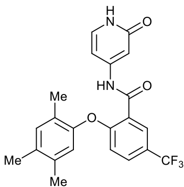
N-(2-oxo-1,2-dihydropyridin-4-yl)-5-(trifluoromethyl)-2-(2,4,5-trimethylphenoxy)benzamide;
