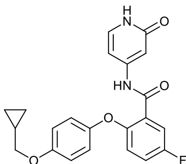
2-(4-(cyclopropylmethoxy)phenoxy)-5-fluoro-N-(2-oxo-1,2-dihydropyridin-4-yl)benzamide;
