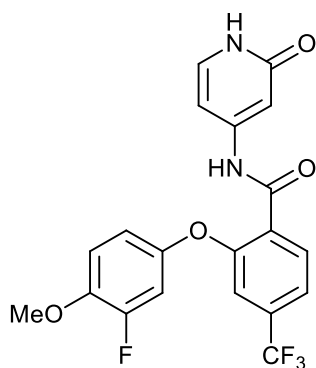
2-(3-fluoro-4-methoxyphenoxy)-N-(2-oxo-1,2-dihydropyridin-4-yl)-4-(trifluoromethyl)benzamide;
