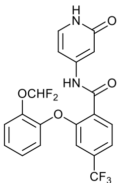
2-(2-(difluoromethoxy)phenoxy)-N-(2-oxo-1,2-dihydropyridin-4-yl)-4-(trifluoromethyl)benzamide;
