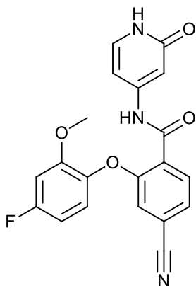
4-cyano-2-(4-fluoro-2-methoxyphenoxy)-N-(2-oxo-1,2-dihydropyridin-4-yl)benzamide;
