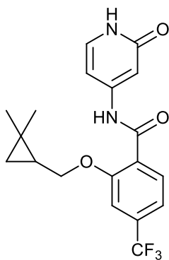
2-((2,2-dimethylcyclopropyl)methoxy)-N-(2-oxo-1,2-dihydropyridin-4-yl)-4-(trifluoromethyl)benzamide;
