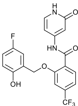
2-((5-fluoro-2-hydroxybenzyl)oxy)-N-(2-oxo-1,2-dihydropyridin-4-yl)-4-(trifluoromethyl)benzamide; and
