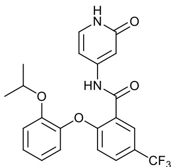
2-(2-isopropoxyphenoxy)-N-(2-oxo-1,2-dihydropyridin-4-yl)-5-(trifluoromethyl)benzamide;
