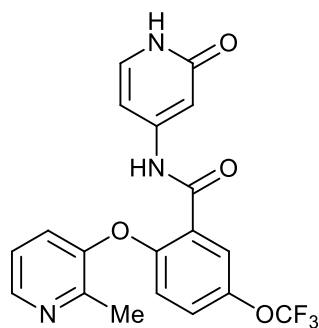
2-((2-methylpyridin-3-yl)oxy)-N-(2-oxo-1,2-dihydropyridin-4-yl)-5-(trifluoromethoxy)benzamide;
