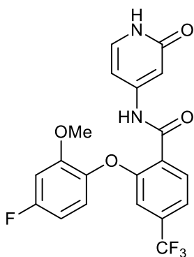
2-(4-fluoro-2-methoxyphenoxy)-N-(2-oxo-1,2-dihydropyridin-4-yl)-4-(trifluoromethyl)benzamide;
