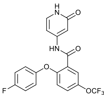
2-(4-fluorophenoxy)-N-(2-oxo-1,2-dihydropyridin-4-yl)-5-(trifluoromethoxy)benzamide;
