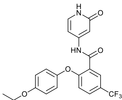
2-(4-ethoxyphenoxy)-N-(2-oxo-1,2-dihydropyridin-4-yl)-5-(trifluoromethyl)benzamide;
