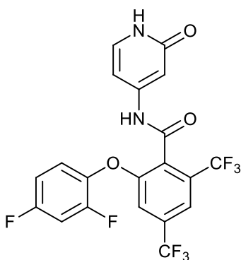
2-(2,4-difluorophenoxy)-N-(2-oxo-1,2-dihydropyridin-4-yl)-4,6-bis(trifluoromethyl)benzamide;
