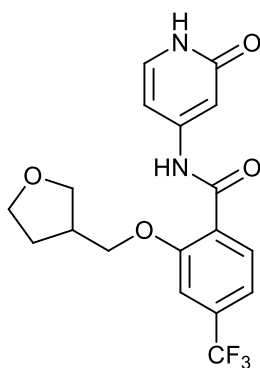
N-(2-oxo-1,2-dihydropyridin-4-yl)-2-((tetrahydrofuran-3-yl)methoxy)-4-(trifluoromethyl)benzamide;
