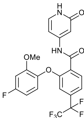
2-(4-fluoro-2-methoxyphenoxy)-N-(2-oxo-1,2-dihydropyridin-4-yl)-4-(perfluoroethyl)benzamide.
