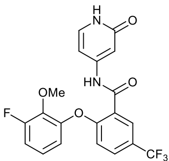
2-(3-fluoro-2-methoxyphenoxy)-N-(2-oxo-1,2-dihydropyridin-4-yl)-5-(trifluoromethyl)benzamide;
