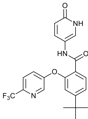
4-(tert-butyl)-N-(6-oxo-1,6-dihydropyridin-3-yl)-2-(((6-(trifluoromethyl)pyridin-3-yl)oxy))benzamide;
