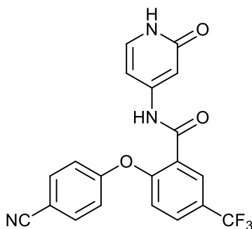
2-(4-cyanophenoxy)-N-(2-oxo-1,2-dihydropyridin-4-yl)-5-(trifluoromethyl)benzamide;
