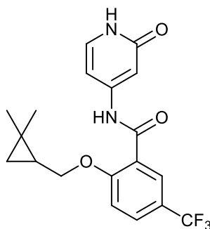
2-((2,2-dimethylcyclopropyl)methoxy)-N-(2-oxo-1,2-dihydropyridin-4-yl)-5-(trifluoromethyl)benzamide;
