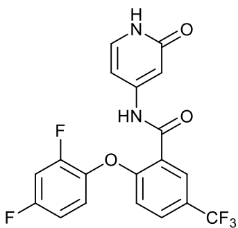
2-(2,4-difluorophenoxy)-N-(2-oxo-1,2-dihydropyridin-4-yl)-5-(trifluoromethyl)benzamide;
