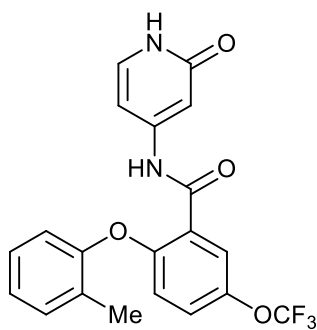
N-(2-oxo-1,2-dihydropyridin-4-yl)-2-(o-tolylloxy)-5-(trifluoromethoxy)benzamide;
