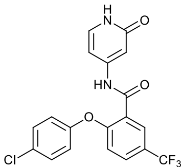
2-(4-chlorophenoxy)-N-(2-oxo-1,2-dihydropyridin-4-yl)-5-(trifluoromethyl)benzamide;
