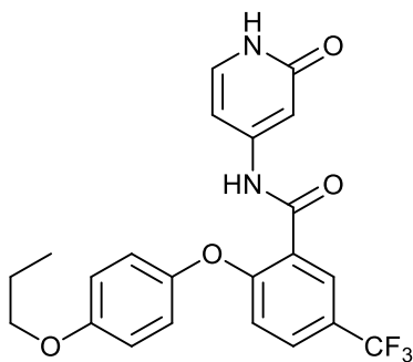
N-(2-oxo-1,2-dihydropyridin-4-yl)-2-(4-propoxyphenoxy)-5-(trifluoromethyl)benzamide;
