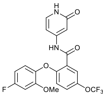
2-(4-fluoro-2-methoxyphenoxy)-N-(2-oxo-1,2-dihydropyridin-4-yl)-5-(trifluoromethoxy)benzamide;
