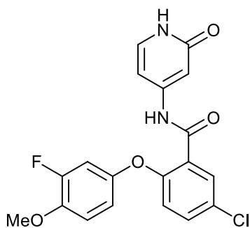
5-chloro-2-(3-fluoro-4-methoxyphenoxy)-N-(2-oxo-1,2-dihydropyridin-4-yl)benzamide;
