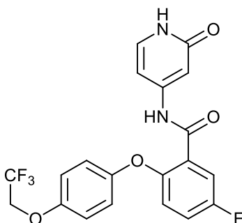
5-fluoro-N-(2-oxo-1,2-dihydropyridin-4-yl)-2-(4-(2,2,2-trifluoroethoxy)phenoxy)benzamide;
