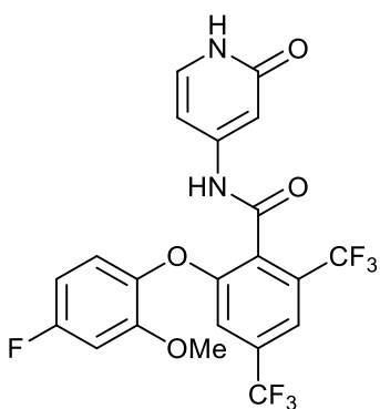
2-(4-fluoro-2-methoxyphenoxy)-N-(2-oxo-1,2-dihydropyridin-4-yl)-4,6-bis(trifluoromethyl)benzamide;
