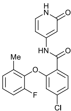
4-chloro-2-(2-fluoro-6-methylphenoxy)-N-(2-oxo-1,2-dihydropyridin-4-yl)benzamide;
