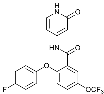
2-(4-fluorophenoxy)-N-(2-oxo-1,2-dihydropyridin-4-yl)-5-(trifluoromethoxy)benzamide;
