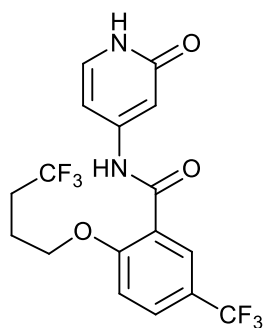
N-(2-oxo-1,2-dihydropyridin-4-yl)-2-(4,4,4-trifluorobutoxy)-5-(trifluoromethyl)benzamide;
