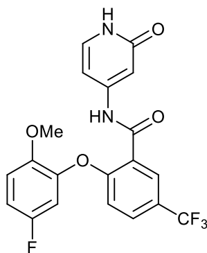
2-(5-fluoro-2-methoxyphenoxy)-N-(2-oxo-1,2-dihydropyridin-4-yl)-5-(trifluoromethyl)benzamide;
