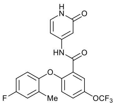
2-(4-fluoro-2-methylphenoxy)-N-(2-oxo-1,2-dihydropyridin-4-yl)-5-(trifluoromethoxy)benzamide;
