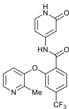
2-((2-methylpyridin-3-yl)oxy)-N-(2-oxo-1,2-dihydropyridin-4-yl)-4-(trifluoromethyl)benzamide;
