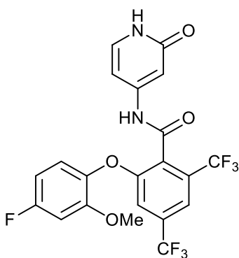
2-(4-fluoro-2-methoxyphenoxy)-N-(2-oxo-1,2-dihydropyridin-4-yl)-4,6-bis(trifluoromethyl)benzamide;
