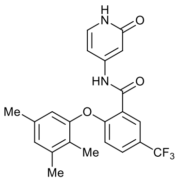
N-(2-oxo-1,2-dihydropyridin-4-yl)-5-(trifluoromethyl)-2-(2,3,5-trimethylphenoxy)benzamide;
