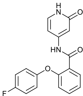
2-(4-fluorophenoxy)-N-(2-oxo-1,2-dihydropyridin-4-yl)benzamide;
