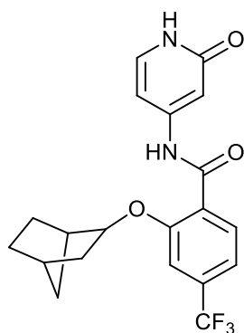
2-(bicyclo[2.2.1]heptan-2-yloxy)-N-(2-oxo-1,2-dihydropyridin-4-yl)-4-(trifluoromethyl)benzamide;
