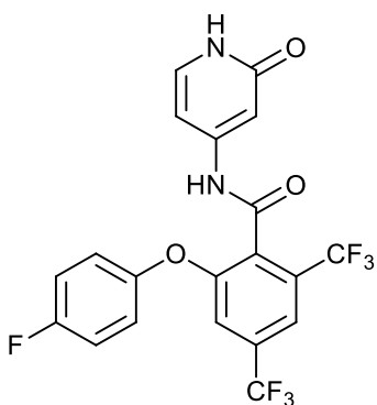
2-(4-fluorophenoxy)-N-(2-oxo-1,2-dihydropyridin-4-yl)-4,6-bis(trifluoromethyl)benzamide;
