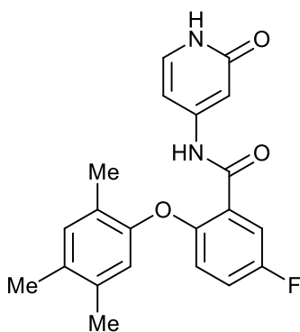
5-fluoro-N-(2-oxo-1,2-dihydropyridin-4-yl)-2-(2,4,5-trimethylphenoxy)benzamide;
