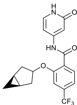
2-((1R,5S)-bicyclo[3.1.0]hexan-3-yloxy)-N-(2-oxo-1,2-dihydropyridin-4-yl)-4-(trifluoromethyl)benzamide;
