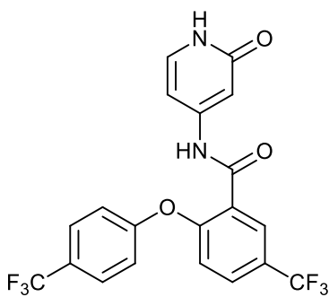
N-(2-oxo-1,2-dihydropyridin-4-yl)-5-(trifluoromethyl)-2-(4-(trifluoromethyl)phenoxy)benzamide;
