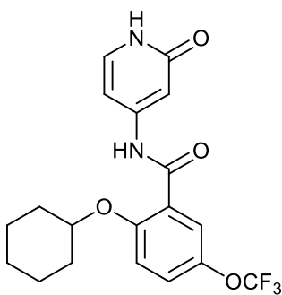
2-(cyclohexyloxy)-N-(2-oxo-1,2-dihydropyridin-4-yl)-5-(trifluoromethoxy)benzamide;
