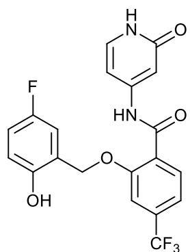
2-((5-fluoro-2-hydroxybenzyl)oxy)-N-(2-oxo-1,2-dihydropyridin-4-yl)-4-(trifluoromethyl)benzamide; and
