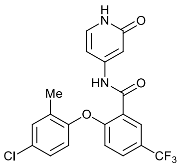
2-(4-chloro-2-methylphenoxy)-N-(2-oxo-1,2-dihydropyridin-4-yl)-5-(trifluoromethyl)benzamide;
