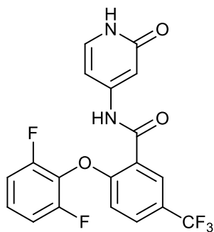
2-(2,6-difluorophenoxy)-N-(2-oxo-1,2-dihydropyridin-4-yl)-5-(trifluoromethyl)benzamide;
