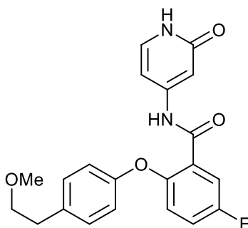
5-fluoro-2-(4-(2-methoxyethyl)phenoxy)-N-(2-oxo-1,2-dihydropyridin-4-yl)benzamide;
