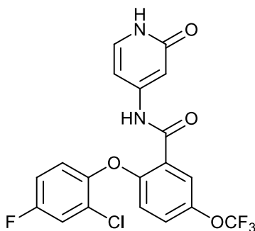
2-(2-chloro-4-fluorophenoxy)-N-(2-oxo-1,2-dihydropyridin-4-yl)-5-(trifluoromethoxy)benzamide;
