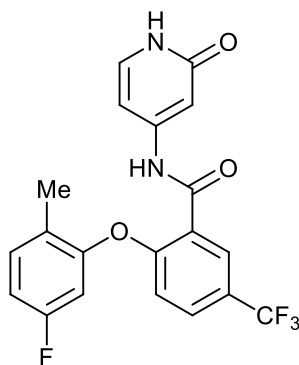
2-(5-fluoro-2-methylphenoxy)-N-(2-oxo-1,2-dihydropyridin-4-yl)-5-(trifluoromethyl)benzamide;
