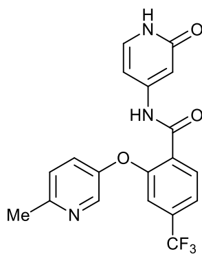
2-((6-methylpyridin-3-yl)oxy)-N-(2-oxo-1,2-dihydropyridin-4-yl)-4-(trifluoromethyl)benzamide;
