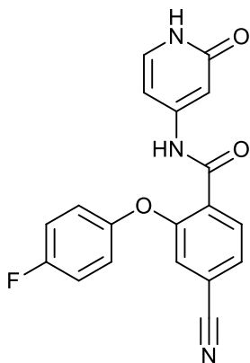
4-cyano-2-(4-fluorophenoxy)-N-(2-oxo-1,2-dihydropyridin-4-yl)benzamide;
