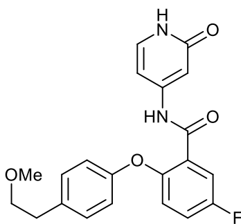
5-fluoro-2-(4-(2-methoxyethyl)phenoxy)-N-(2-oxo-1,2-dihydropyridin-4-yl)benzamide;
