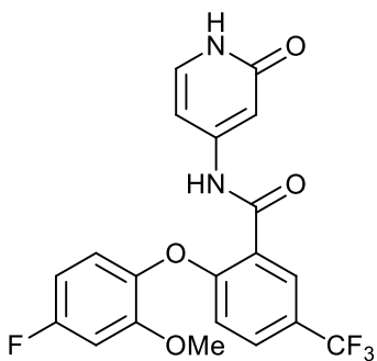
2-(4-fluoro-2-methoxyphenoxy)-N-(2-oxo-1,2-dihydropyridin-4-yl)-5-(trifluoromethyl)benzamide;
