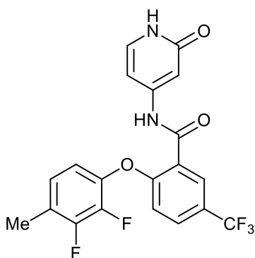
2-(2,3-difluoro-4-methylphenoxy)-N-(2-oxo-1,2-dihydropyridin-4-yl)-5-(trifluoromethyl)benzamide;
