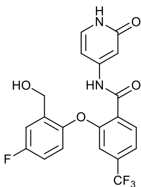
2-(4-fluoro-2-(hydroxymethyl)phenoxy)-N-(2-oxo-1,2-dihydropyridin-4-yl)-4-(trifluoromethyl)benzamide;
