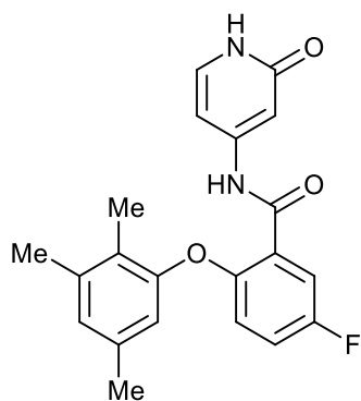
5-fluoro-N-(2-oxo-1,2-dihydropyridin-4-yl)-2-(2,3,5-trimethylphenoxy)benzamide;
