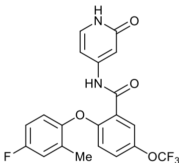
2-(4-fluoro-2-methylphenoxy)-N-(2-oxo-1,2-dihydropyridin-4-yl)-5-(trifluoromethoxy)benzamide;
