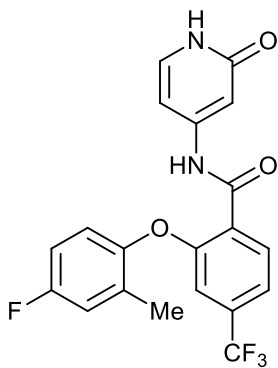
N-(2-oxo-1,2-dihydropyridin-4-yl)-2-phenoxy-4-(trifluoromethyl)benzamide;
