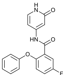
5-fluoro-N-(2-oxo-1,2-dihydropyridin-4-yl)-2-phenoxybenzamide;
