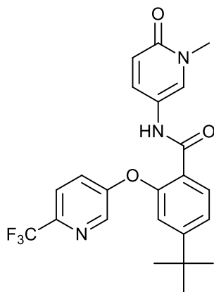
4-(tert-butyl)-N-(1-methyl-6-oxo-1,6-dihydropyridin-3-yl)-2-((6-(trifluoromethyl)pyridin-3-yl)oxy)benzamide;
