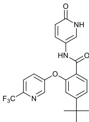
4-(tert-butyl)-N-(6-oxo-1,6-dihydropyridin-3-yl)-2-((6-(trifluoromethyl)pyridin-3-yl)oxy)benzamide;
