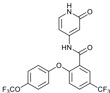
N-(2-oxo-1,2-dihydropyridin-4-yl)-2-(4-(trifluoromethoxy)phenoxy)-5-(trifluoromethyl)benzamide;
