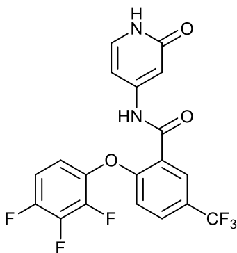
N-(2-oxo-1,2-dihydropyridin-4-yl)-5-(trifluoromethyl)-2-(2,3,4-trifluorophenoxy)benzamide;
