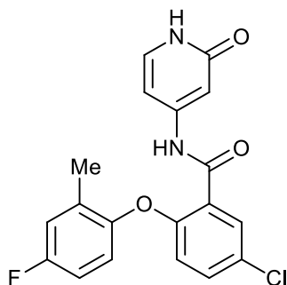
5-chloro-2-(4-fluoro-2-methylphenoxy)-N-(2-oxo-1,2-dihydropyridin-4-yl)benzamide;
