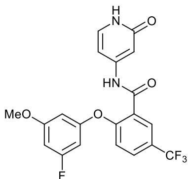
2-(3-fluoro-5-methoxyphenoxy)-N-(2-oxo-1,2-dihydropyridin-4-yl)-5-(trifluoromethyl)benzamide;
