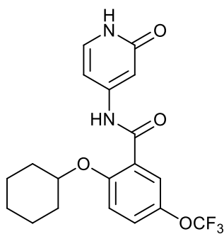
2-(cyclohexyloxy)-N-(2-oxo-1,2-dihydropyridin-4-yl)-5-(trifluoromethoxy)benzamide;
