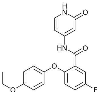
2-(4-ethoxyphenoxy)-5-fluoro-N-(2-oxo-1,2-dihydropyridin-4-yl)benzamide;
