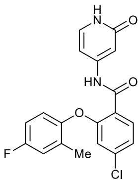
4-chloro-2-(4-fluoro-2-methylphenoxy)-N-(2-oxo-1,2-dihydropyridin-4-yl)benzamide.
