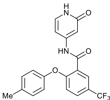
N-(2-oxo-1,2-dihydropyridin-4-yl)-2-(p-tolyloxy)-5-(trifluoromethyl)benzamide;
