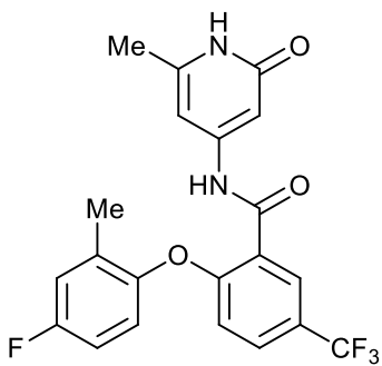
2-(4-fluoro-2-methylphenoxy)-N-(6-methyl-2-oxo-1,2-dihydropyridin-4-yl)-5-(trifluoromethyl)benzamide;
