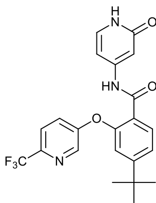
4-(tert-butyl)-N-(2-oxo-1,2-dihydropyridin-4-yl)-2-(((6-(trifluoromethyl)pyridin-3-yl)oxy))benzamide;
