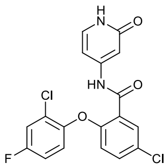
5-chloro-2-(2-chloro-4-fluorophenoxy)-N-(2-oxo-1,2-dihydropyridin-4-yl)benzamide;
