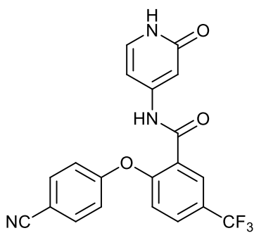
2-(4-cyanophenoxy)-N-(2-oxo-1,2-dihydropyridin-4-yl)-5-(trifluoromethyl)benzamide;
