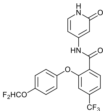
2-(4-(difluoromethoxy)phenoxy)-N-(2-oxo-1,2-dihydropyridin-4-yl)-4-(trifluoromethyl)benzamide;
