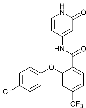
2-(4-chlorophenoxy)-N-(2-oxo-1,2-dihydropyridin-4-yl)-4-(trifluoromethyl)benzamide;
