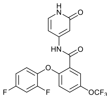
2-(2,4-difluorophenoxy)-N-(2-oxo-1,2-dihydropyridin-4-yl)-5-(trifluoromethoxy)benzamide;
