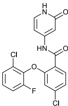
4-chloro-2-(2-chloro-6-fluorophenoxy)-N-(2-oxo-1,2-dihydropyridin-4-yl)benzamide;
