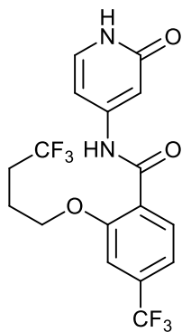
N-(2-oxo-1,2-dihydropyridin-4-yl)-2-(4,4,4-trifluorobutoxy)-4-(trifluoromethyl)benzamide;
