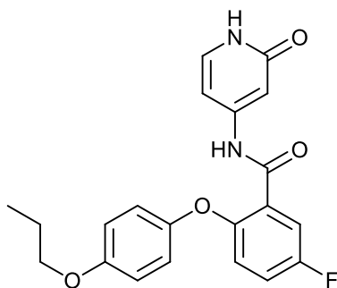
5-fluoro-N-(2-oxo-1,2-dihydropyridin-4-yl)-2-(4-propoxyphenoxy)benzamide;
