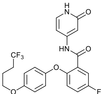
5-fluoro-N-(2-oxo-1,2-dihydropyridin-4-yl)-2-(4-(4,4,4-trifluorobutoxy)phenoxy)benzamide;
