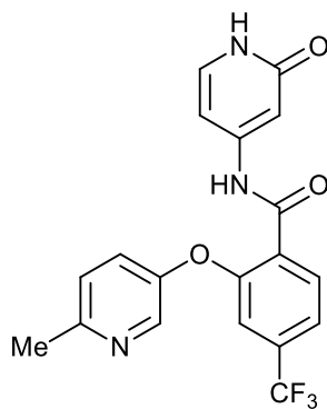
2-((6-methylpyridin-3-yl)oxy)-N-(2-oxo-1,2-dihydropyridin-4-yl)-4-(trifluoromethyl)benzamide;
