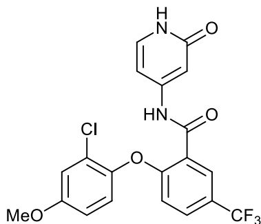
2-(2-chloro-4-methoxyphenoxy)-N-(2-oxo-1,2-dihydropyridin-4-yl)-5-(trifluoromethyl)benzamide;
