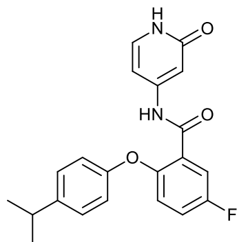
5-fluoro-2-(4-isopropylphenoxy)-N-(2-oxo-1,2-dihydropyridin-4-yl)benzamide;
