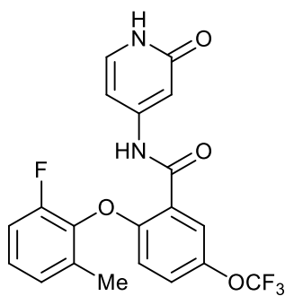
2-(2-fluoro-6-methylphenoxy)-N-(2-oxo-1,2-dihydropyridin-4-yl)-5-(trifluoromethoxy)benzamide;
