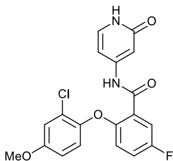
2-(2-chloro-4-methoxyphenoxy)-5-fluoro-N-(2-oxo-1,2-dihydropyridin-4-yl)benzamide;
