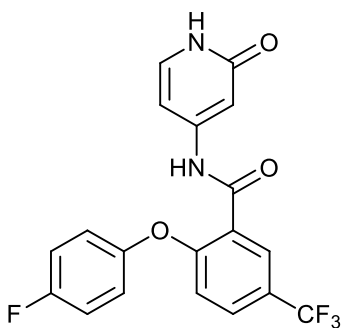
2-(4-fluorophenoxy)-N-(2-oxo-1,2-dihydropyridin-4-yl)-5-(trifluoromethyl)benzamide;
