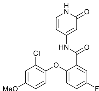
2-(2-chloro-4-methoxyphenoxy)-5-fluoro-N-(2-oxo-1,2-dihydropyridin-4-yl)benzamide;
