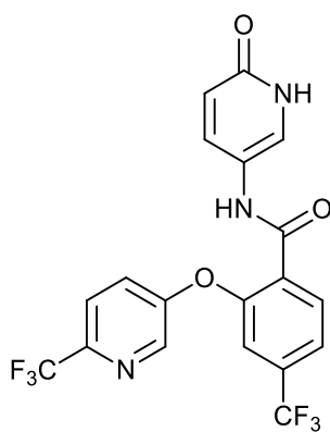
N-(6-oxo-1,6-dihydropyridin-3-yl)-4-(trifluoromethyl)-2-((6-(trifluoromethyl)pyridin-3-yl)oxy)benzamide;
