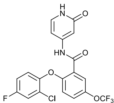
2-(2-chloro-4-fluorophenoxy)-N-(2-oxo-1,2-dihydropyridin-4-yl)-5-(trifluoromethoxy)benzamide;
