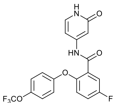
5-fluoro-N-(2-oxo-1,2-dihydropyridin-4-yl)-2-(4-(trifluoromethoxy)phenoxy)benzamide;
