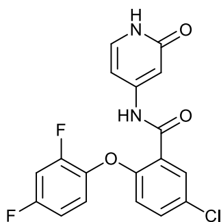
5-chloro-2-(2,4-difluorophenoxy)-N-(2-oxo-1,2-dihydropyridin-4-yl)benzamide;
