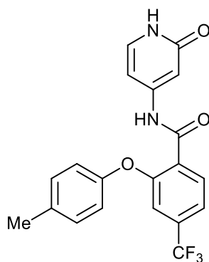
N-(2-oxo-1,2-dihydropyridin-4-yl)-2-(p-tolyloxy)-4-(trifluoromethyl)benzamide;
