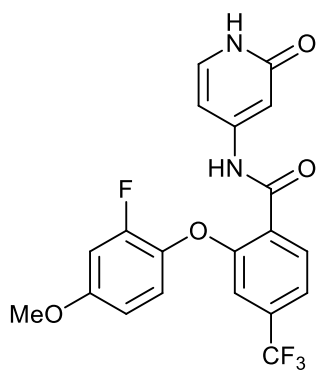
2-(2-fluoro-4-methoxyphenoxy)-N-(2-oxo-1,2-dihydropyridin-4-yl)-4-(trifluoromethyl)benzamide;
