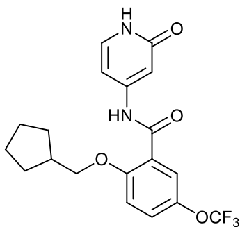
2-(cyclopentylmethoxy)-N-(2-oxo-1,2-dihydropyridin-4-yl)-5-(trifluoromethoxy)benzamide;
