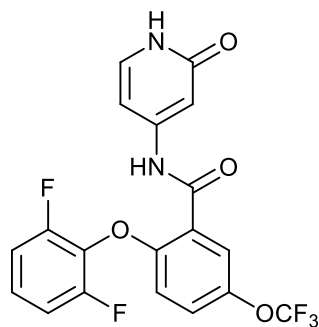
2-(2,6-difluorophenoxy)-N-(2-oxo-1,2-dihydropyridin-4-yl)-5-(trifluoromethoxy)benzamide;
