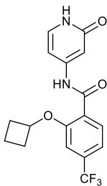
2-cyclobutoxy-N-(2-oxo-1,2-dihydropyridin-4-yl)-4-(trifluoromethyl)benzamide;
