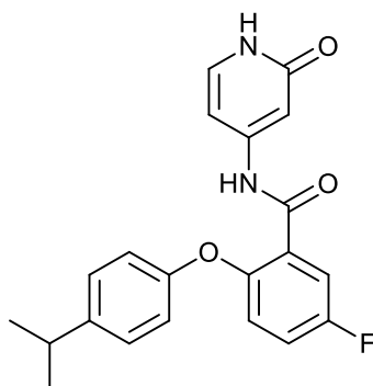
5-fluoro-2-(4-isopropylphenoxy)-N-(2-oxo-1,2-dihydropyridin-4-yl)benzamide;
