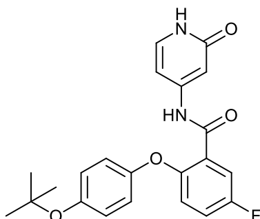
2-(4-(tert-butoxy)phenoxy)-5-fluoro-N-(2-oxo-1,2-dihydropyridin-4-yl)benzamide;
