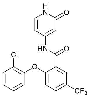
2-(2-chlorophenoxy)-N-(2-oxo-1,2-dihydropyridin-4-yl)-5-(trifluoromethyl)benzamide;
