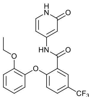
2-(2-ethoxyphenoxy)-N-(2-oxo-1,2-dihydropyridin-4-yl)-5-(trifluoromethyl)benzamide;
