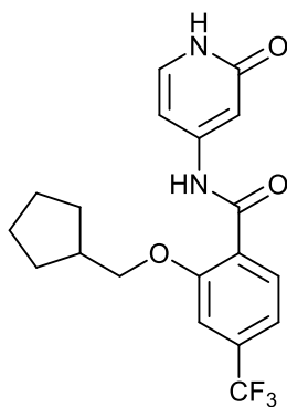
2-(cyclopentylmethoxy)-N-(2-oxo-1,2-dihydropyridin-4-yl)-4-(trifluoromethyl)benzamide;
