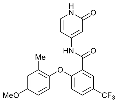
2-(4-methoxy-2-methylphenoxy)-N-(2-oxo-1,2-dihydropyridin-4-yl)-5-(trifluoromethyl)benzamide;
