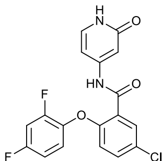
5-chloro-2-(2,4-difluorophenoxy)-N-(2-oxo-1,2-dihydropyridin-4-yl)benzamide;
