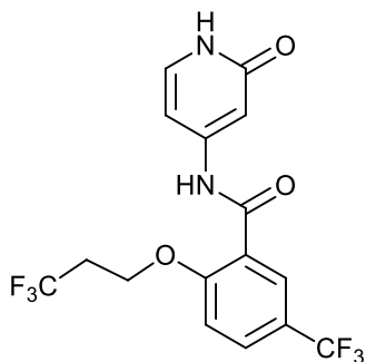
N-(2-oxo-1,2-dihydropyridin-4-yl)-5-(trifluoromethyl)-2-(3,3,3-trifluoropropoxy)benzamide;
