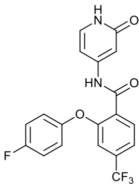
2-(4-fluorophenoxy)-N-(2-oxo-1,2-dihydropyridin-4-yl)-4-(trifluoromethyl)benzamide;
