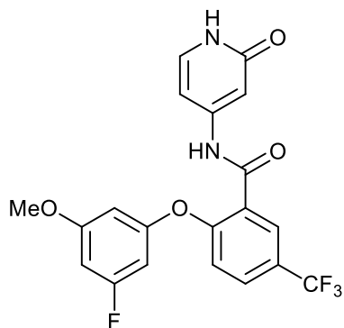
2-(3-fluoro-5-methoxyphenoxy)-N-(2-oxo-1,2-dihydropyridin-4-yl)-5-(trifluoromethyl)benzamide;
