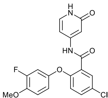
5-chloro-2-(3-fluoro-4-methoxyphenoxy)-N-(2-oxo-1,2-dihydropyridin-4-yl)benzamide;
