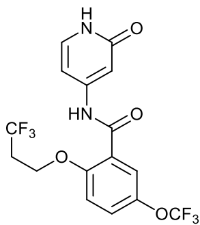
N-(2-oxo-1,2-dihydropyridin-4-yl)-5-(trifluoromethoxy)-2-(3,3,3-trifluoropropoxy)benzamide;
