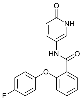
2-(4-fluorophenoxy)-N-(6-oxo-1,6-dihydropyridin-3-yl)benzamide;
