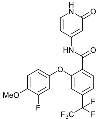
2-(3-fluoro-4-methoxyphenoxy)-N-(2-oxo-1,2-dihydropyridin-4-yl)-4-(perfluoroethyl)benzamide;
