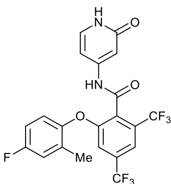
2-(4-fluoro-2-methylphenoxy)-N-(2-oxo-1,2-dihydropyridin-4-yl)-4,6-bis(trifluoromethyl)benzamide;
