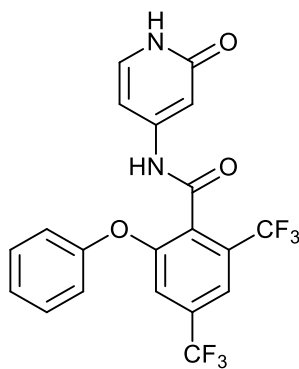
N-(2-oxo-1,2-dihydropyridin-4-yl)-2-phenoxy-4,6-bis(trifluoromethyl)benzamide;
