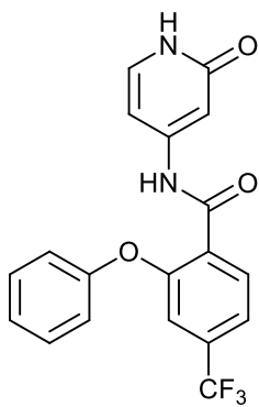
N-(2-oxo-1,2-dihydropyridin-4-yl)-2-phenoxy-4-(trifluoromethyl)benzamide;
