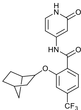
2-(bicyclo[2.2.1]heptan-2-yloxy)-N-(2-oxo-1,2-dihydropyridin-4-yl)-4-(trifluoromethyl)benzamide;
