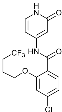
4-chloro-N-(2-oxo-1,2-dihydropyridin-4-yl)-2-(4,4,4-trifluorobutoxy)benzamide;
