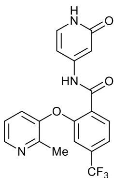
2-((2-methylpyridin-3-yl)oxy)-N-(2-oxo-1,2-dihydropyridin-4-yl)-4-(trifluoromethyl)benzamide;
