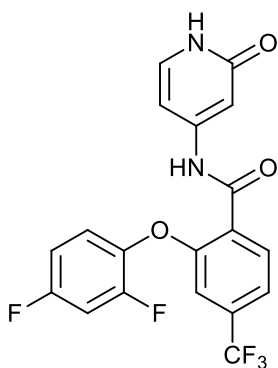
2-(2,4-difluorophenoxy)-N-(2-oxo-1,2-dihydropyridin-4-yl)-4-(trifluoromethyl)benzamide;
