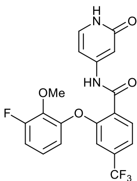
2-(3-fluoro-2-methoxyphenoxy)-N-(2-oxo-1,2-dihydropyridin-4-yl)-4-(trifluoromethyl)benzamide;
