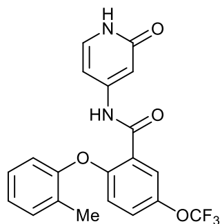
N-(2-oxo-1,2-dihydropyridin-4-yl)-2-(o-tolyloxy)-5-(trifluoromethoxy)benzamide;
