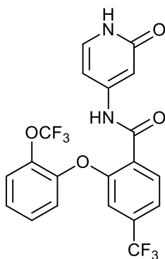
N-(2-oxo-1,2-dihydropyridin-4-yl)-2-(2-(trifluoromethoxy)phenoxy)-4-(trifluoromethyl)benzamide;
