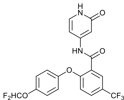
2-(4-(difluoromethoxy)phenoxy)-N-(2-oxo-1,2-dihydropyridin-4-yl)-5-(trifluoromethyl)benzamide;
