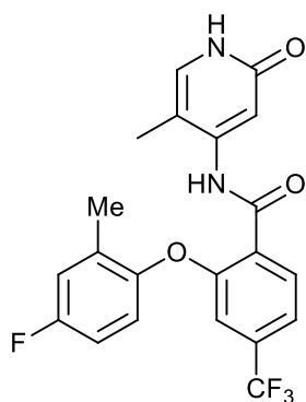
2-(4-fluoro-2-methylphenoxy)-N-(5-methyl-2-oxo-1,2-dihydropyridin-4-yl)-4-(trifluoromethyl)benzamide;
