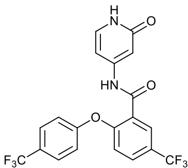
N-(2-oxo-1,2-dihydropyridin-4-yl)-5-(trifluoromethyl)-2-(4-(trifluoromethyl)phenoxy)benzamide;
