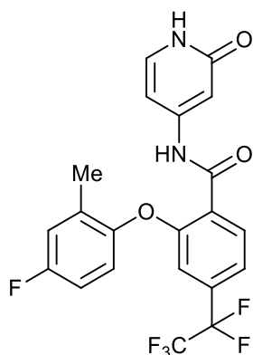
2-(4-fluoro-2-methylphenoxy)-N-(2-oxo-1,2-dihydropyridin-4-yl)-4-(perfluoroethyl)benzamide;
