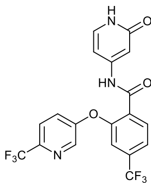
N-(2-oxo-1,2-dihydropyridin-4-yl)-4-(trifluoromethyl)-2-((6-(trifluoromethyl)pyridin-3-yl)oxy)benzamide;
