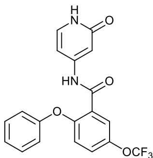
N-(2-oxo-1,2-dihydropyridin-4-yl)-2-phenoxy-5-(trifluoromethoxy)benzamide;
