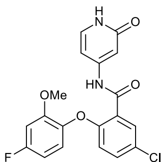
5-chloro-2-(4-fluoro-2-methoxyphenoxy)-N-(2-oxo-1,2-dihydropyridin-4-yl)benzamide;
