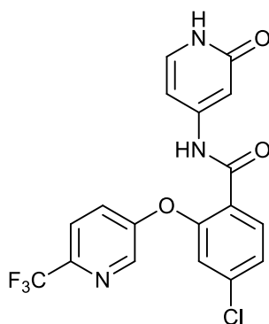
4-chloro-N-(2-oxo-1,2-dihydropyridin-4-yl)-2-((6-(trifluoromethyl)pyridin-3-yl)oxy)benzamide;
