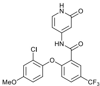
2-(2-chloro-4-methoxyphenoxy)-N-(2-oxo-1,2-dihydropyridin-4-yl)-5-(trifluoromethyl)benzamide;
