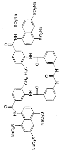
Suramin
