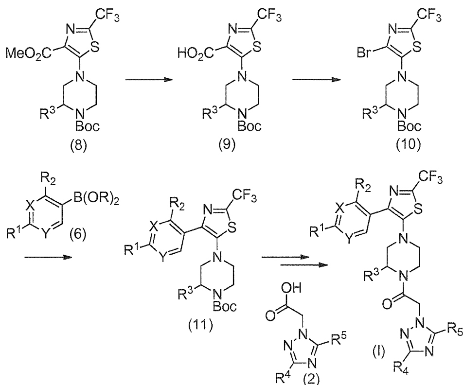
Scheme 3
