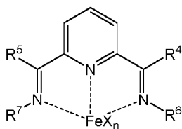
Structure PBIFe III
