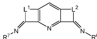
Structure PBI IV
