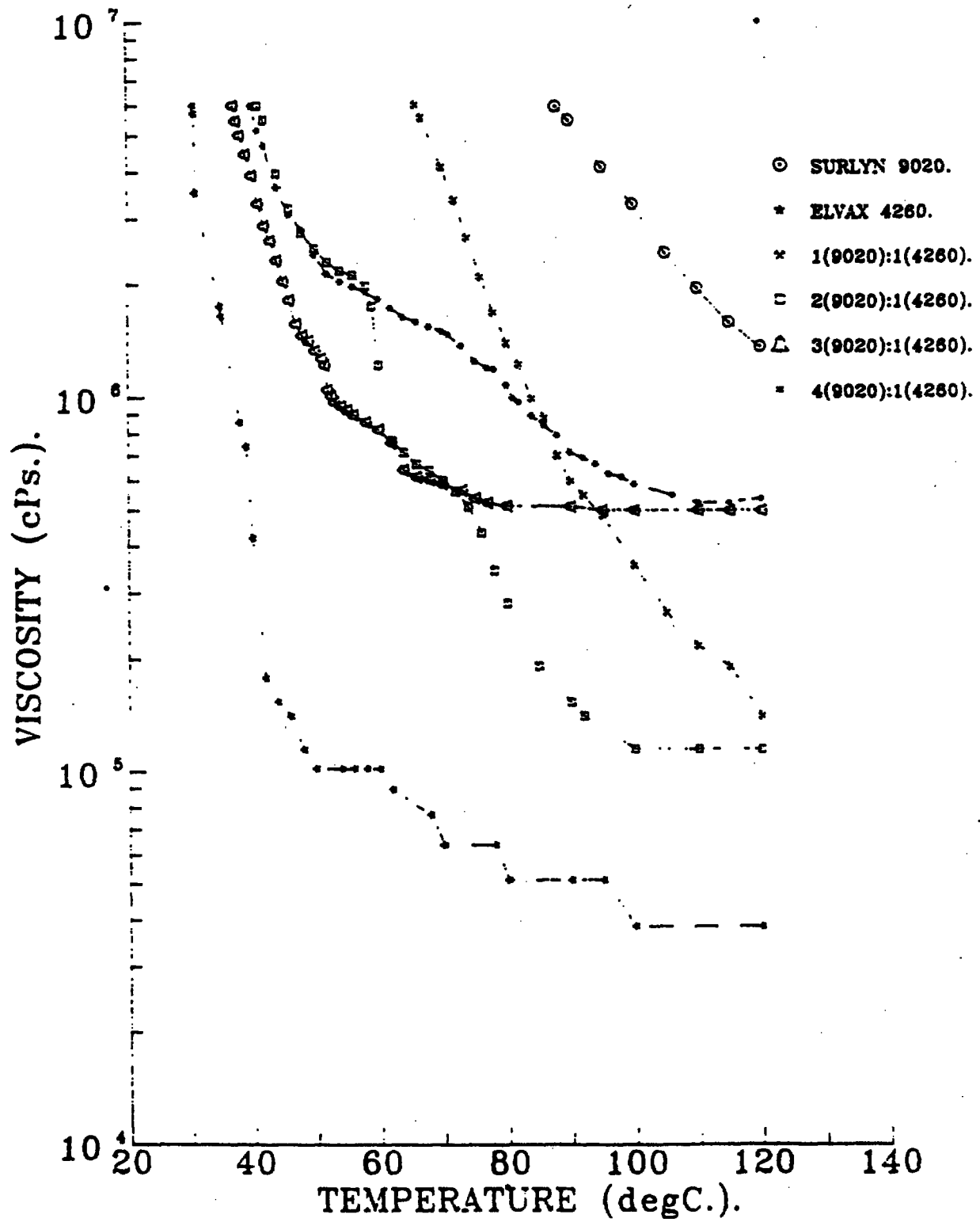
FIG 2: SURLYN 9020-ELVAX 4260 BLENDS 40per.NVS. in ISOPAR L. (cooling curve).
