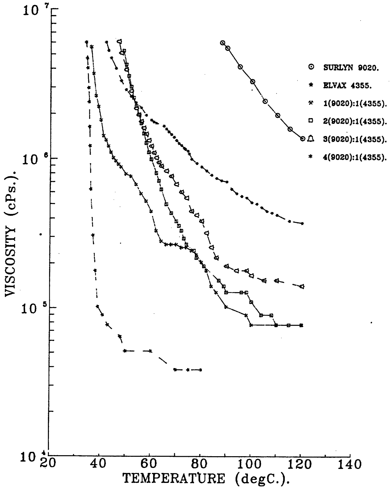
FIG 3: SURLYN 9020-ELVAX 4355 BLENDS 40per.NVS. in ISOPAR L. (cooling curve).
