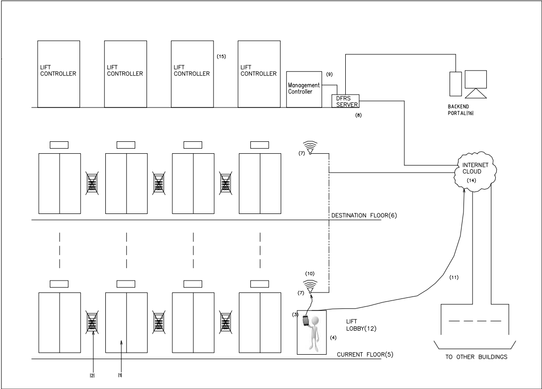
FIG 1: SYSTEM CONFIGURATION
