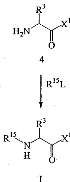
Reaction Scheme 4.
