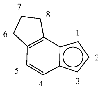
3,6,7,8-tetrahydro- as -indacenyl or 6,7,8-trihydro- as -indacenyl or as -indacenyl
