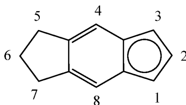
1,5,6,7-tetrahydro- s -indacenyl or 5,6,7-trihydro- s -indacenyl or s -indacenyl
