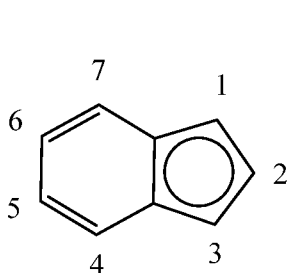
indenyl
