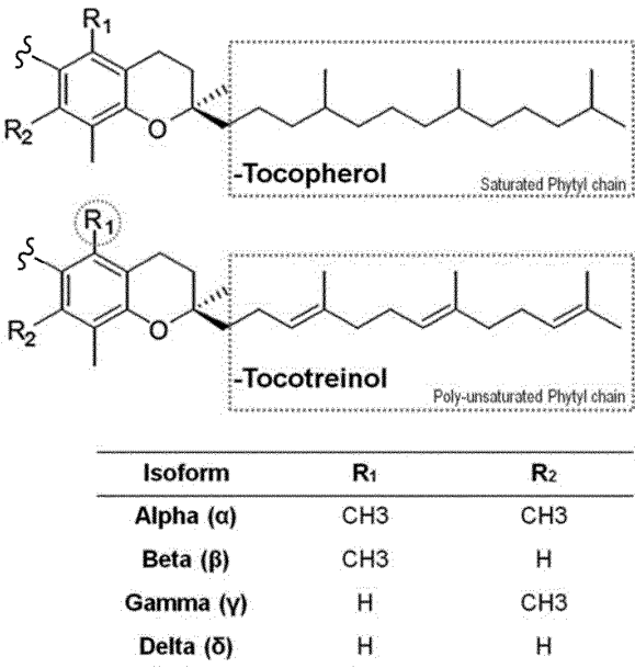
Scheme 1: Derivatives of tocopherol have a saturated phytyl chain, whereas derivatives of tocotreinol have a poly-unsaturated phytyl chain. For both, derivatives of tocopherol and tocotreinol, the isoforms are defined by R 1 and R 2 , which are selected from CH 3 and H. Thus, as shown, if e.g. R 1 is CH 3 and R 2 is CH 3 , the resulting derivative is the alpha isoform of tocopherol and tocotreinol, respectively (referred to as derivative of alpha-tocopherol and alpha-tocotreinol, respectively). The OH-group is of course not present in the derivatives since this is the point of attachment, as shown in the two structures on the left.
