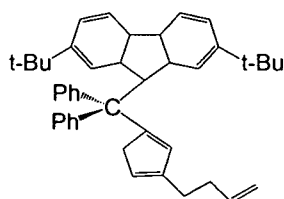
Mixture of isomers L-4
