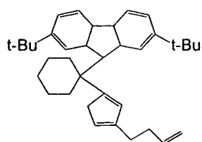
Mixture of isomers L-1
