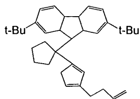
Mixture of isomers L-2
