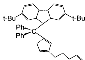
Mixture of isomers L-5
