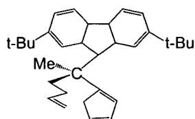
Mixture of isomers L-3
