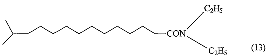
N,N-Diethyl-13-methyl-tetradecanamide
