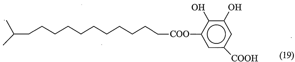
(5-Carboxy-2,3-dihydroxy phenyl)-13-methyl-tetradecanate
