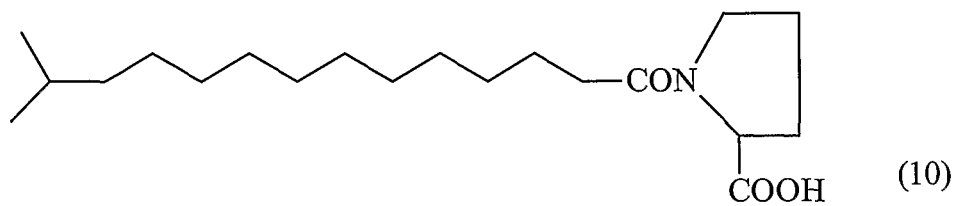
N-(13-Methyl-tetradecanoyl)-L-proline
