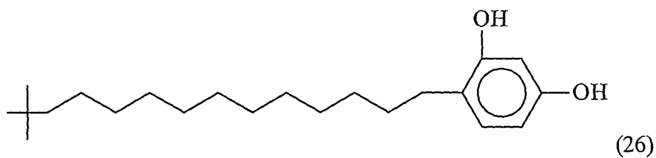
(13,13-Dimethyl tetradecyl)-2,4-dihydroxy phenyl
