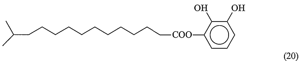
(2,3-Dihydroxy phenyl)-13-methyl-tetradecanate
