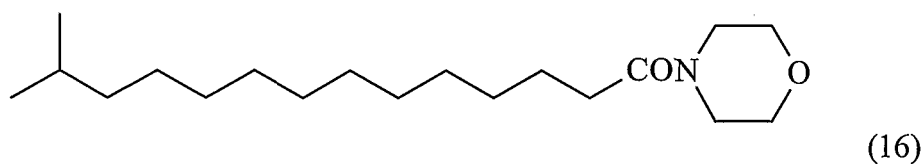
N-(13-Methyl-tetradecanoyl) morpholine
