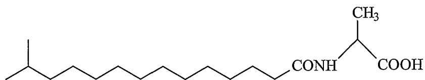
N-(13-Methyl-tetradecanoyl)glycine
