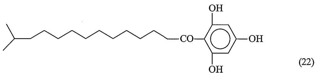
(2,4,6-Trihydroxy phenyl)-12-methyl tridecanone
