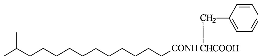
N-(13-Methyl-tetradecanoyl)-L-alanine
