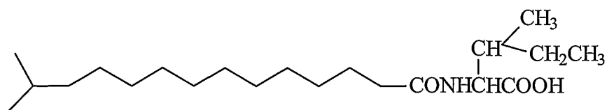
N-(13-Methyl-tetradecanoyl)-L-isoleucine
