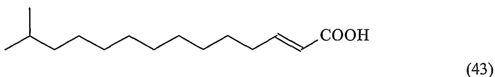
15-Methyl-2-hexadecenoic acid
