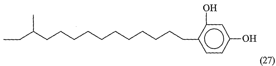
(12-Methyl tetradecyl)-2,4-dihydroxy phenyl
