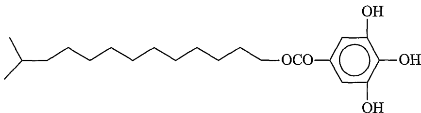
13-Methyltetradecyl-3,4,5-trihydroxy benzoate
