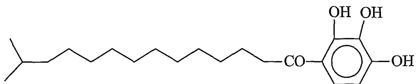
(2,3,4-Trihydroxy phenyl)-12-methyl tridecanone
