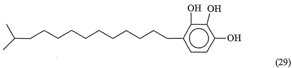
(13-Methyl tetradecyl)-2,4,6-trihydroxy phenyl
