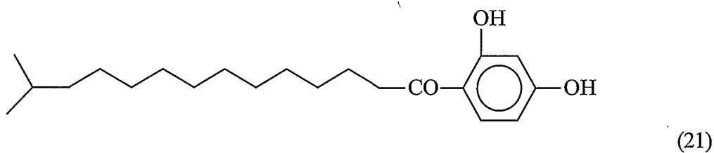
(2,4-dihydroxy phenyl)-12-methyl tridecanone
