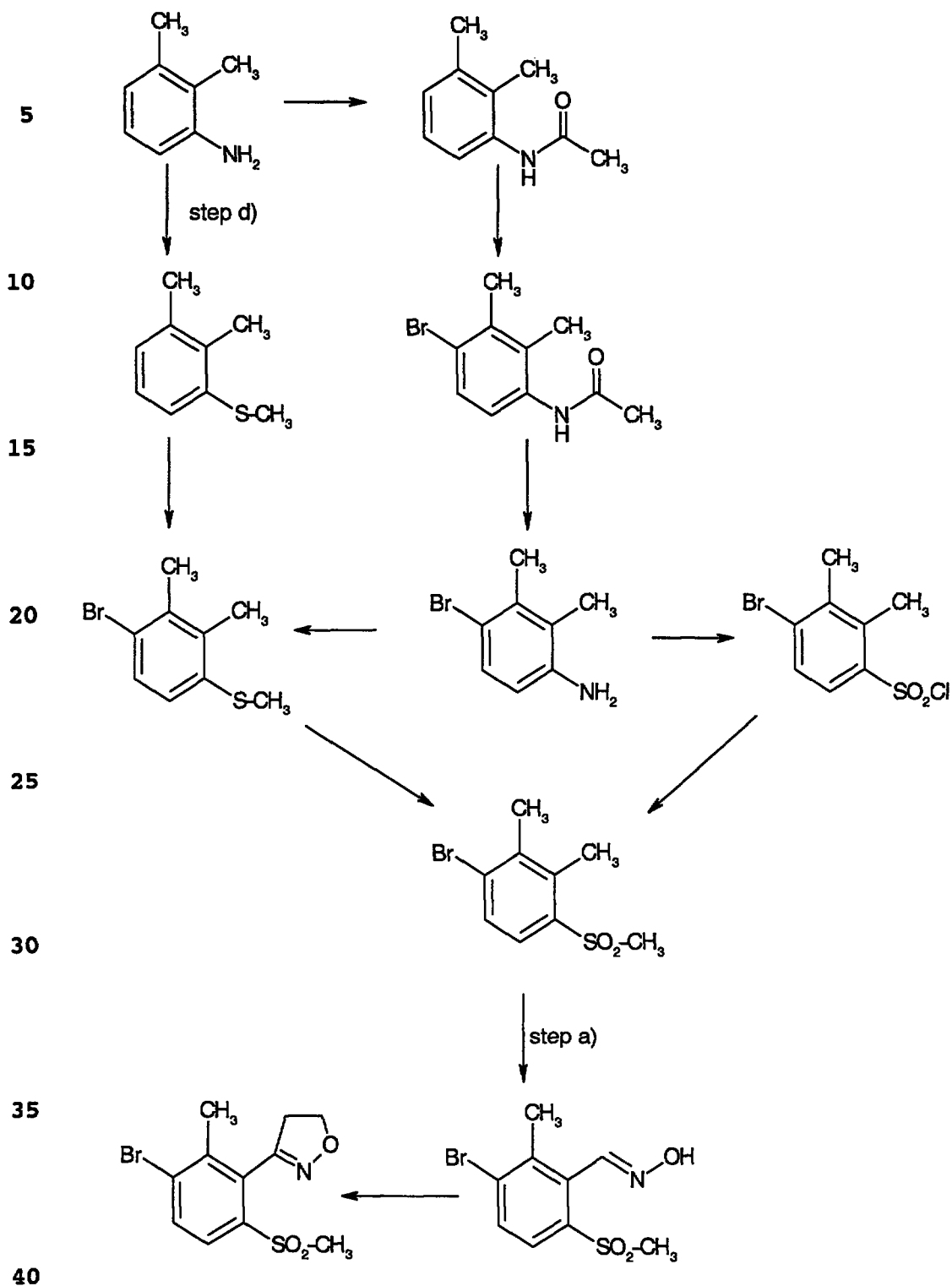
Scheme 4:
