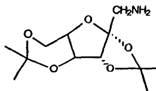
FORMULA XIX
