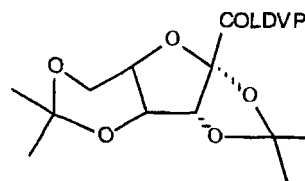
FORMULA XXI
