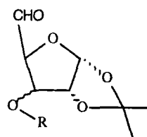
FORMULA VII
