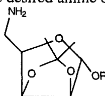
FORMULA XIV
