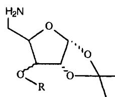
FORMULA X
