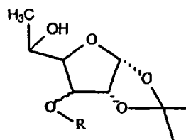
FORMULA V
