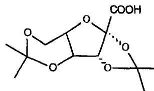
FORMULA XV
