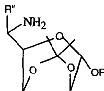
FORMULA XII
