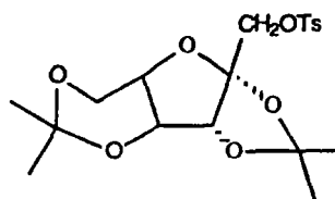
FORMULA XVII
