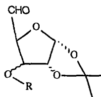
FORMULA VII
