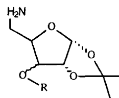
FORMULA X
