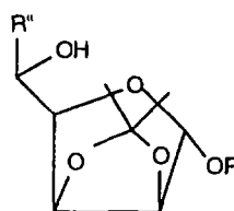
FORMULA XI
