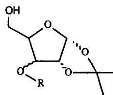
FORMULA IX
