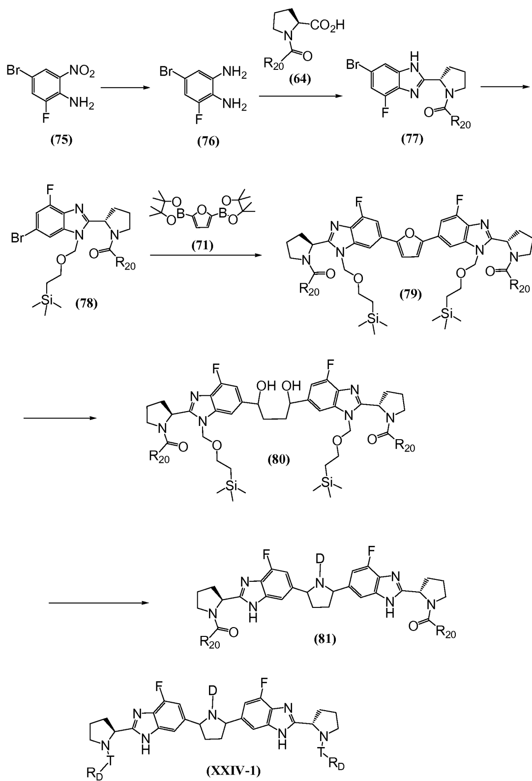
Scheme XXIV
