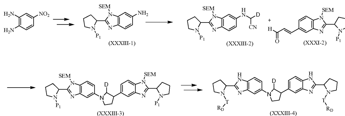
Scheme XXXIII
