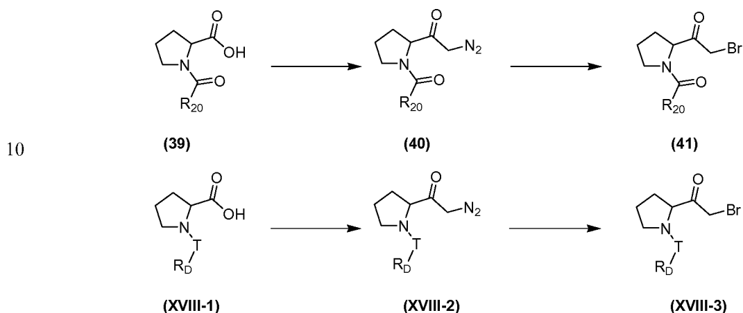
Scheme XVIII
