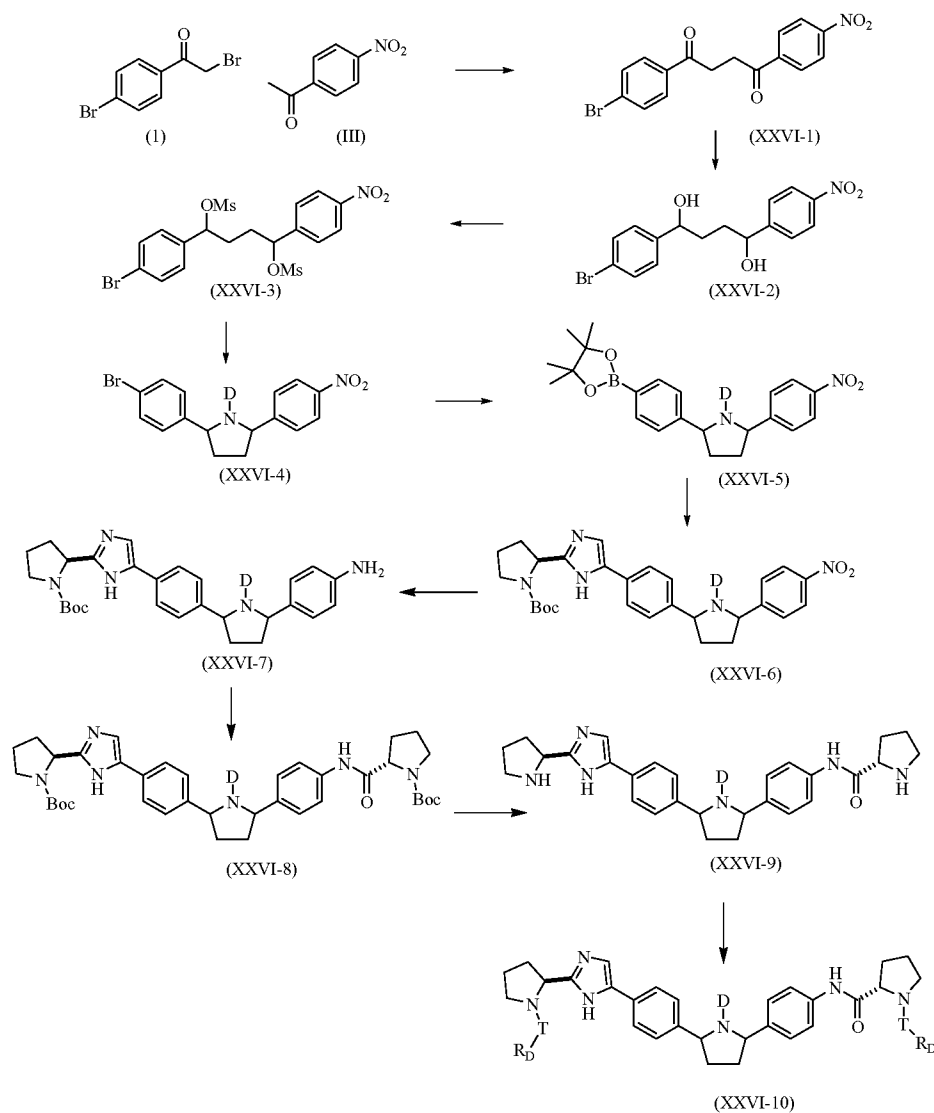
Scheme XXVI
