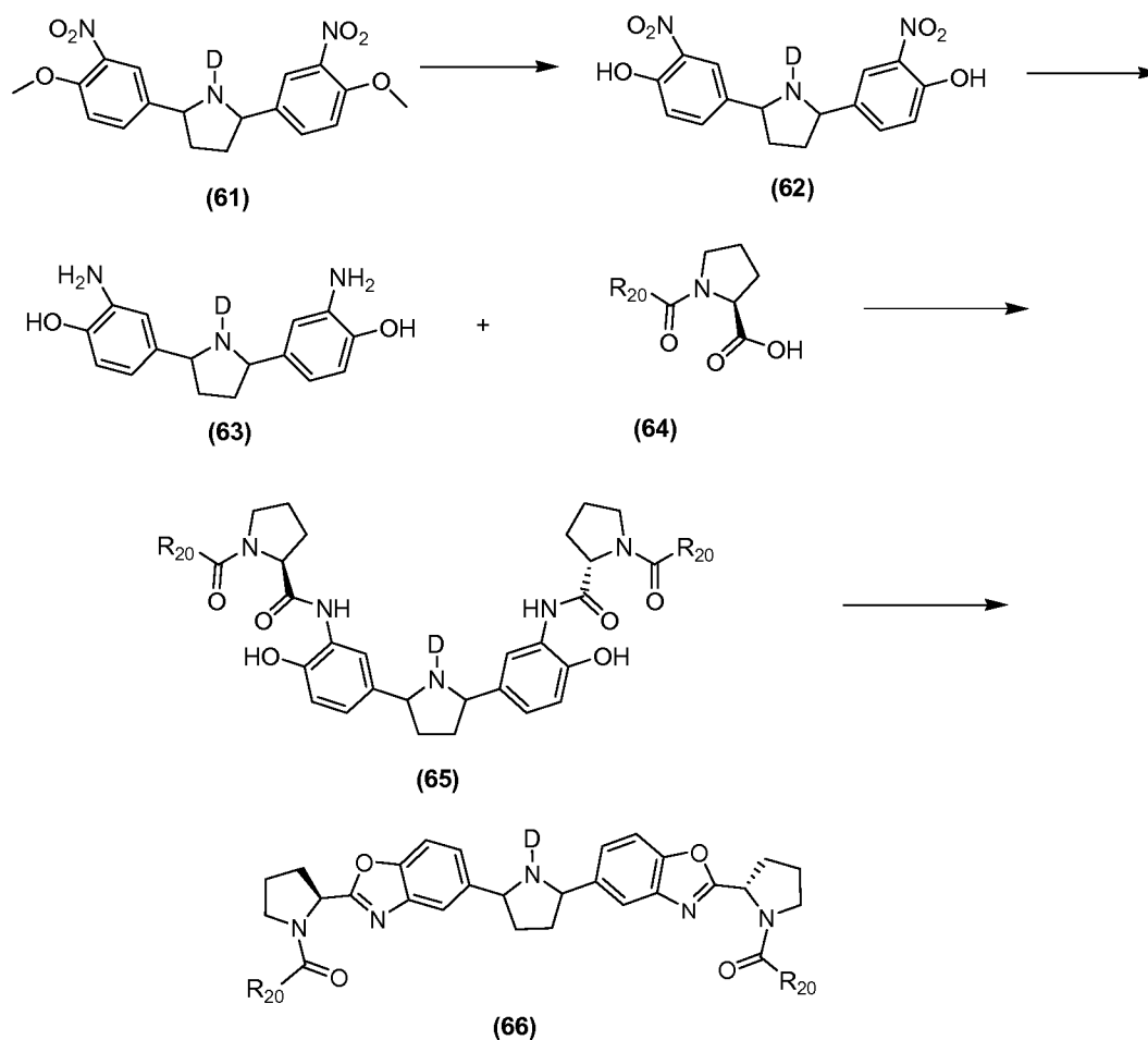
Scheme XXII
