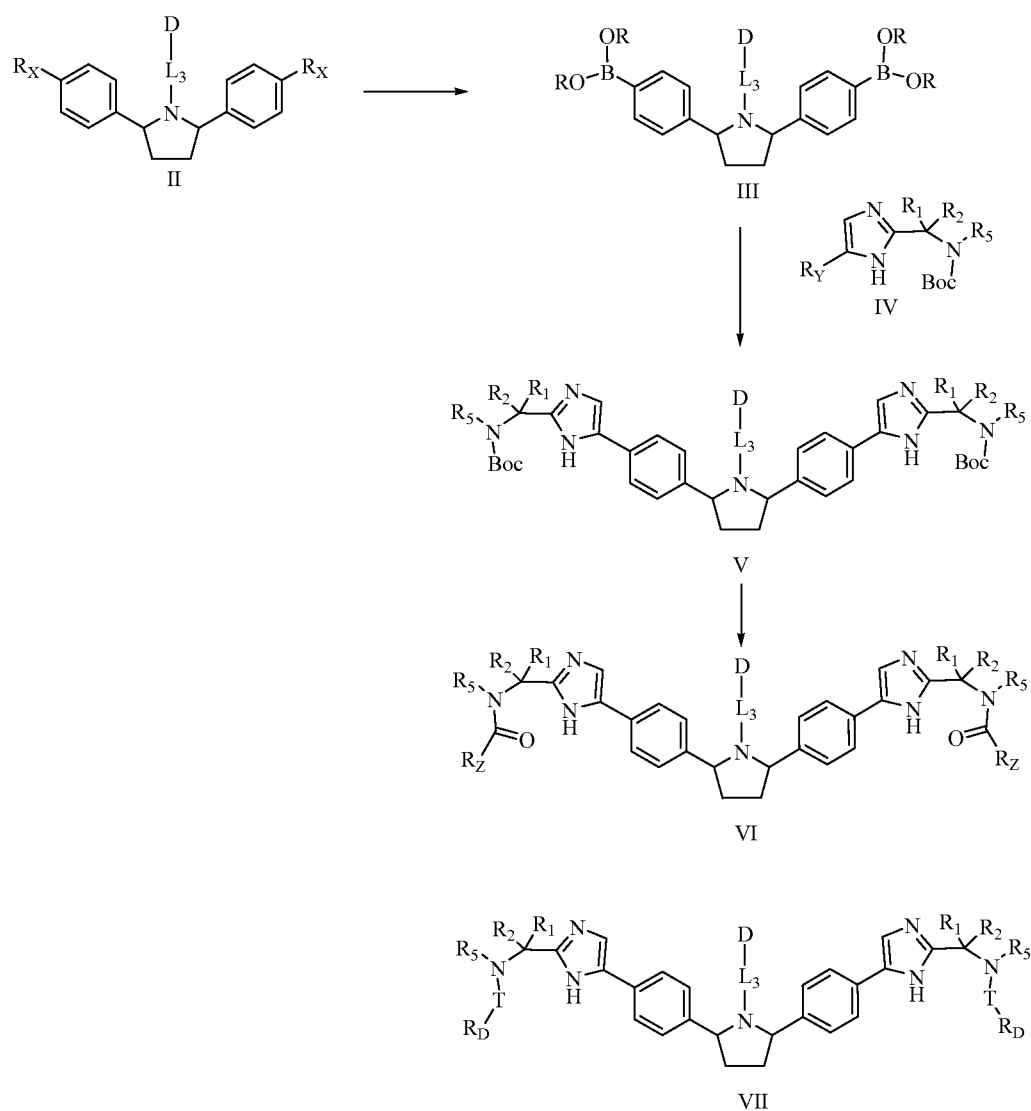
Scheme VII
