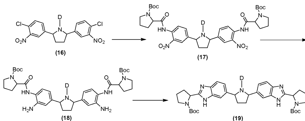
Scheme XIII
