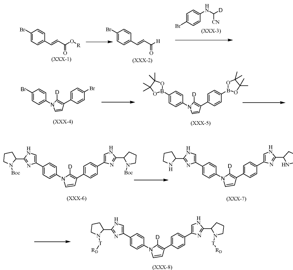
Scheme XXX
