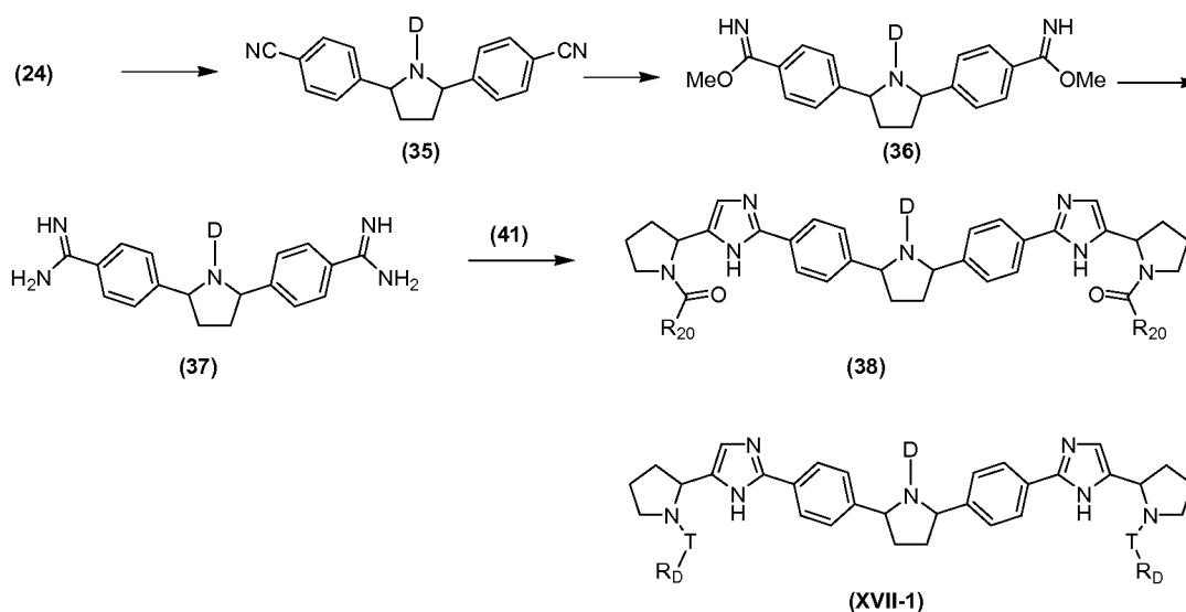
Scheme XVII
