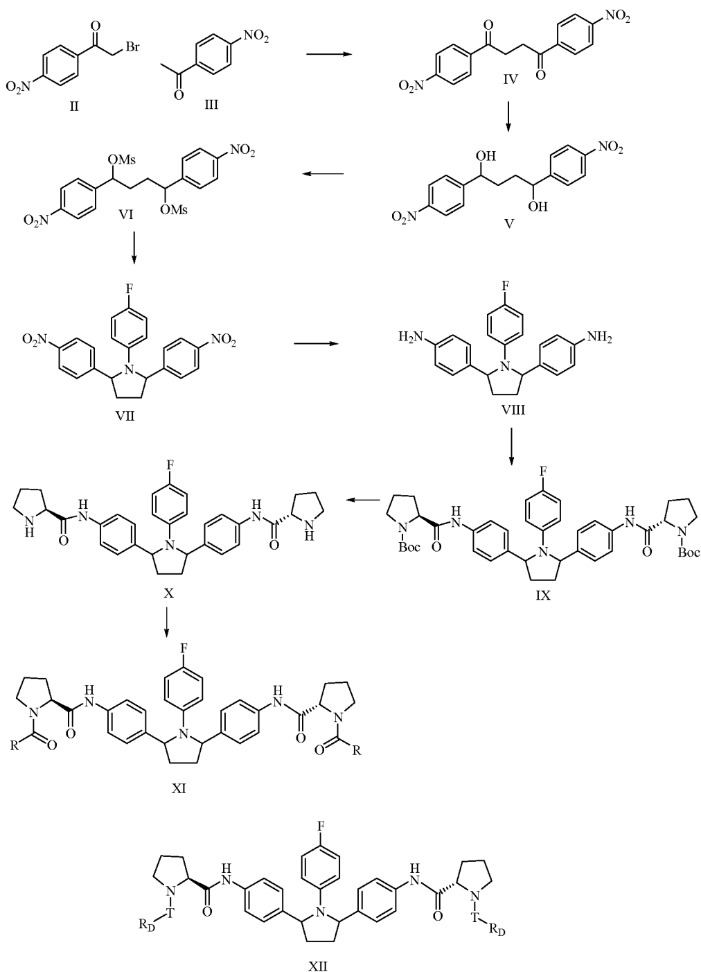
Scheme II
