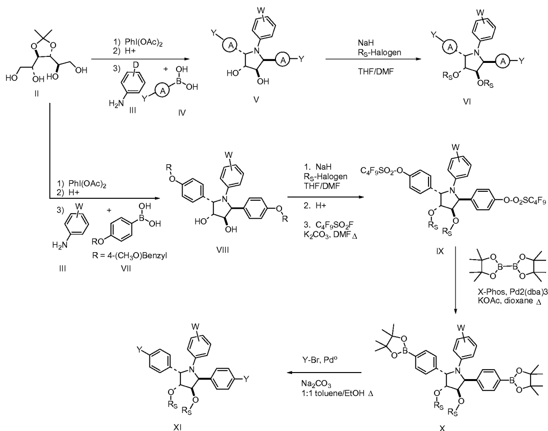
Scheme VIII
