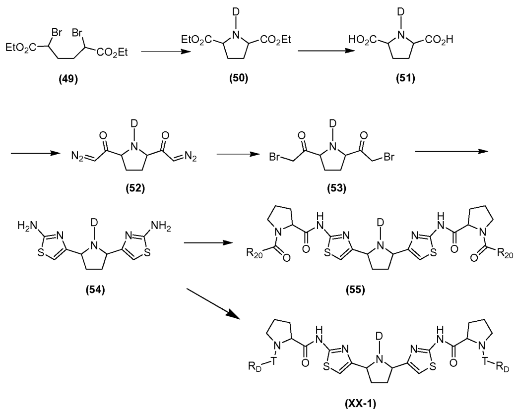
Scheme XX
