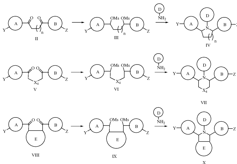
Scheme I
