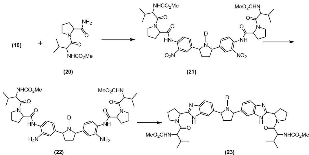
Scheme XIV
