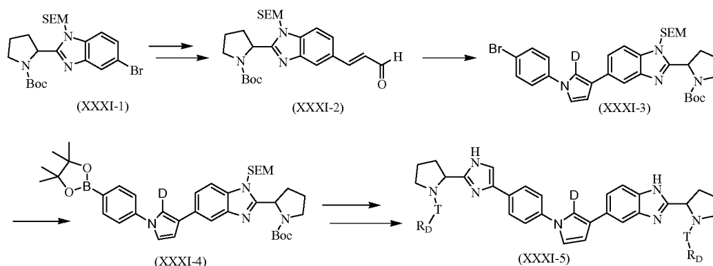
Scheme XXXI
