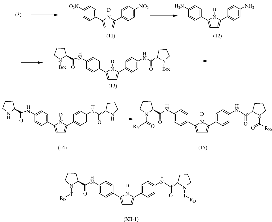
Scheme XII
