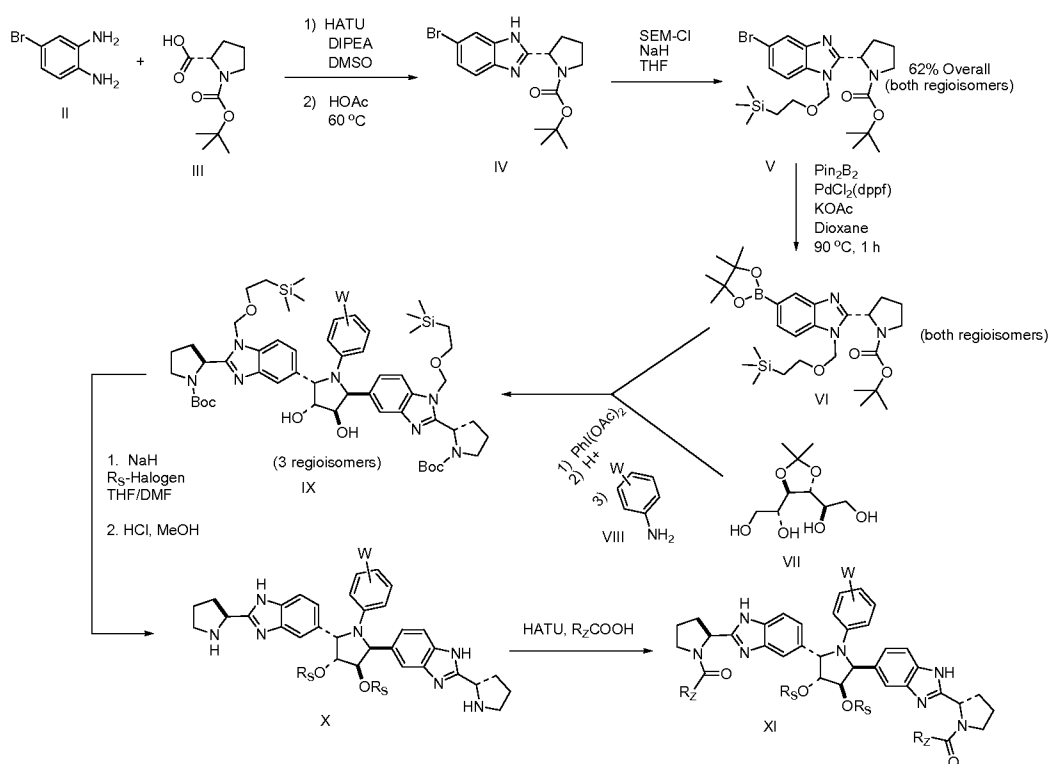
Scheme IX
