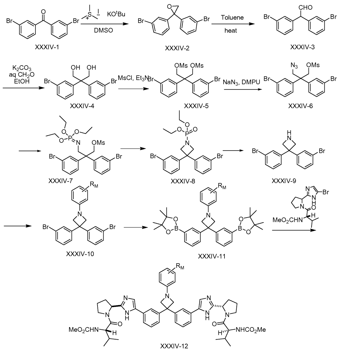
Scheme XXXIV
