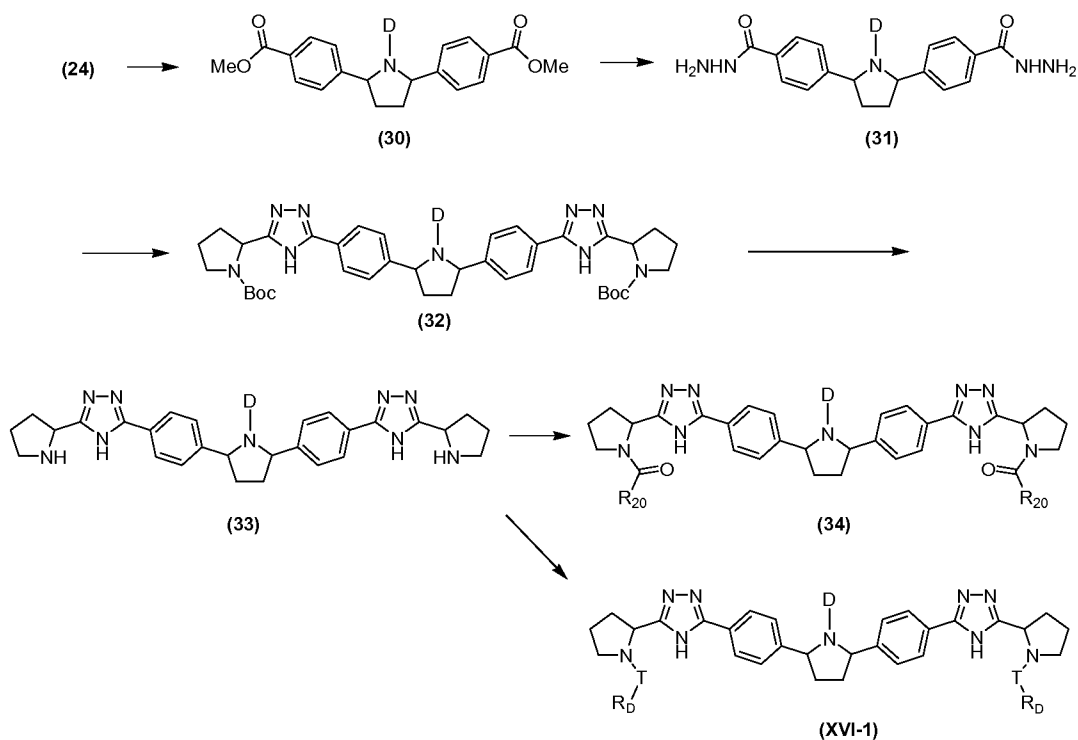
Scheme XVI
