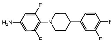
(4-(4-(3,4-difluorophenyl)piperidin-1-yl)-3,5-difluoroaniline
