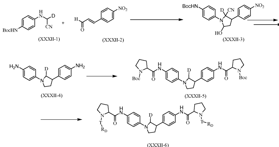
Scheme XXXII
