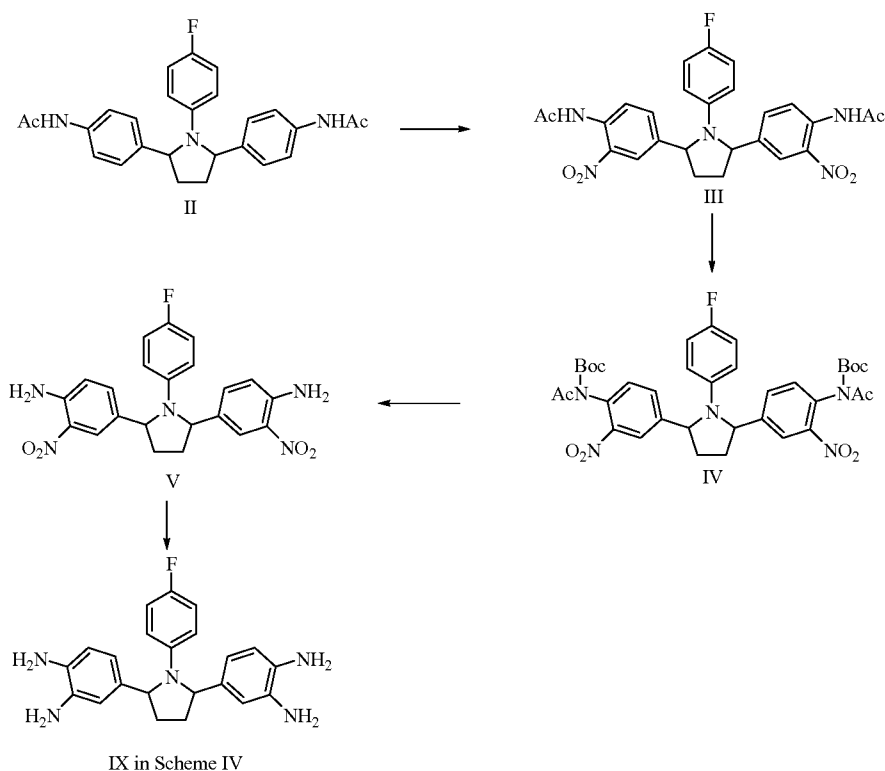
Scheme V
