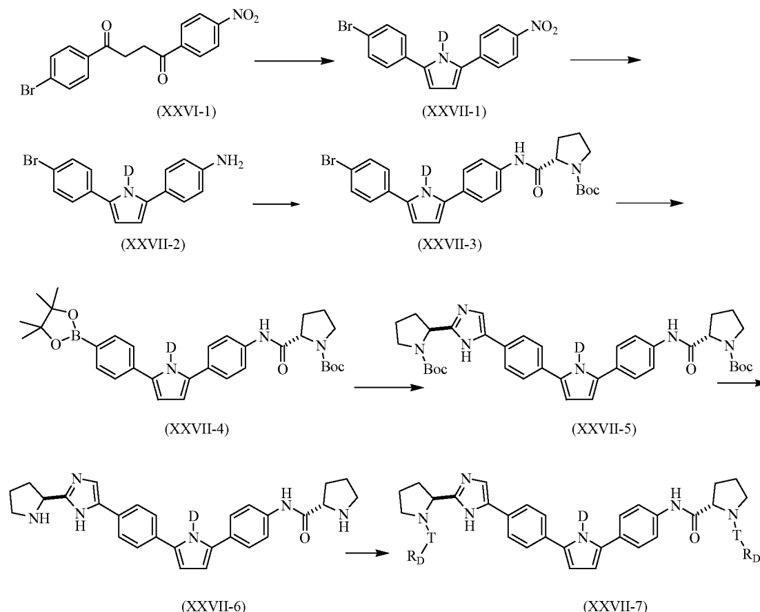
Scheme XXVII
