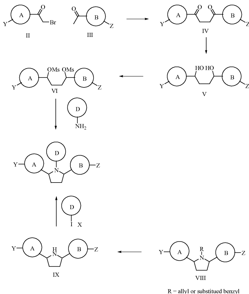
Scheme III
