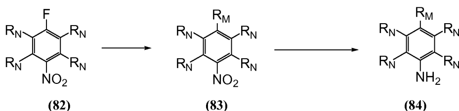
Scheme XXV
