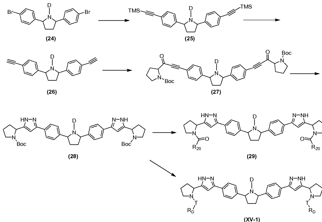
Scheme XV
