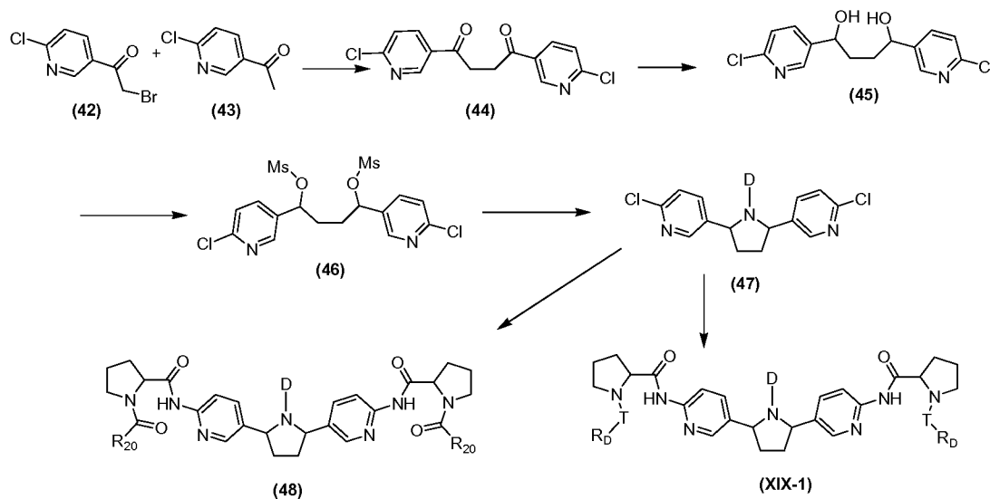
Scheme XIX
