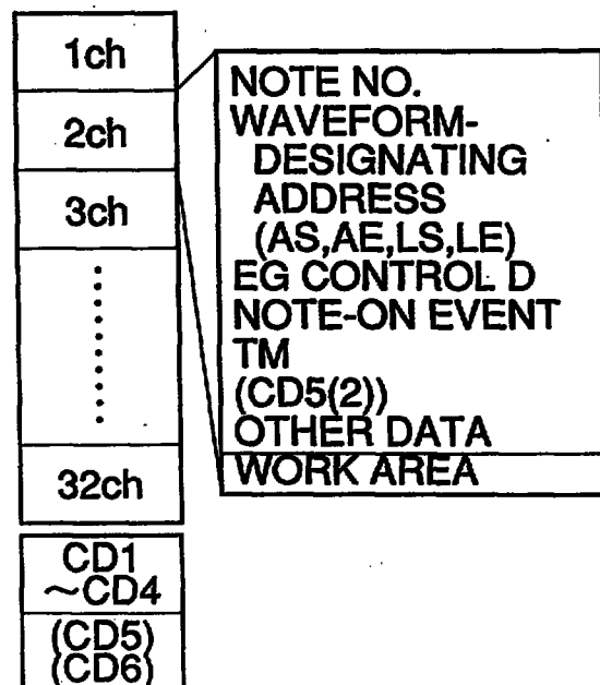
FIG.14D TONE GENERATOR REGISTER
