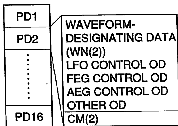
FIG.2A TONE COLOR DATA
