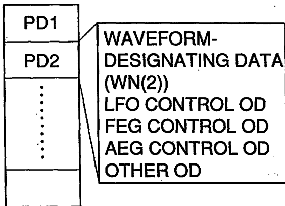
FIG.14A TONE COLOR DATA
