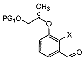
[Chemical Formula 7]
