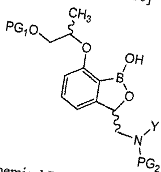
[Chemical Formula 10]
