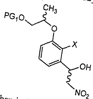
[Chemical Formula 12]
