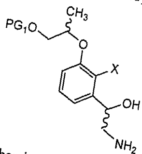
[Chemical Formula 13]
