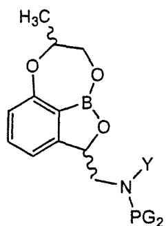
[Chemical Formula 1]
