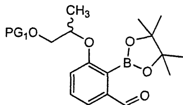
[Chemical Formula 8]
