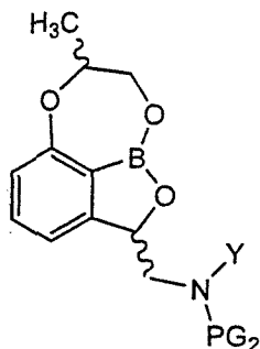
[Chemical Formula 1]
