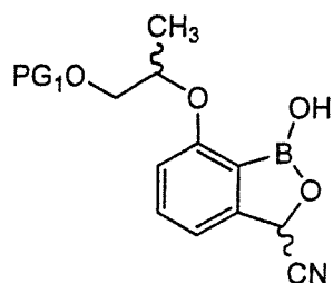
[Chemical Formula 9]
