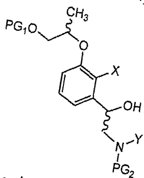
[Chemical Formula 14]
