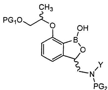
[Chemical Formula 11]
