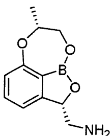
[Chemical Formula 3]
