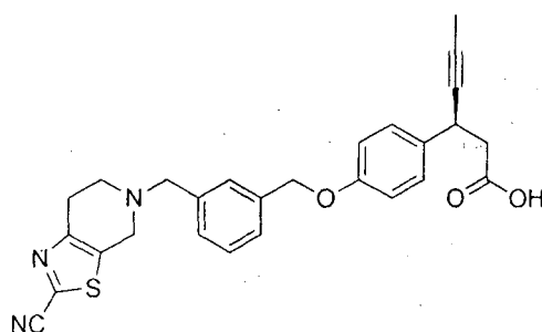
5 (3S)-3-(4-((3-((4-phenyl-6,7-dihydrothieno[3,2-c]pyridin-5(4H)-yl)methyl)benzyl)oxy)phenyl)hex-4-ynoic acid
