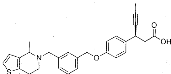
(3S)-3-(4-((3-((4-methyl-6,7-dihydrothieno[3,2-c]pyridin-5(4H)-yl)methyl)benzyl)oxy)phenyl)hex-4-ynoic acid
