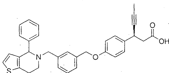
(3S)-3-(4-((3-((4-methyl-6,7-dihydrothieno[3,2-c]pyridin-5(4H)-yl)methyl)benzyl)oxy)phenyl)hex-4-ynoic acid
