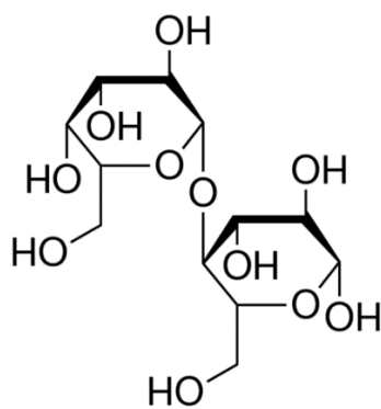
beta-lactose,
