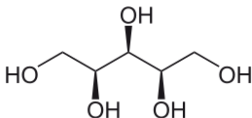
Xylitol,
