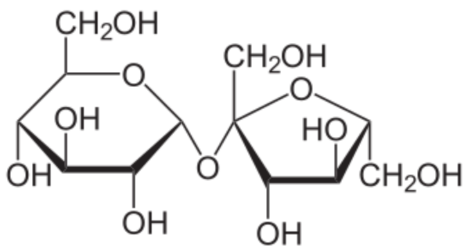
Sucrose,
