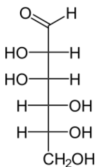
D-Mannose
