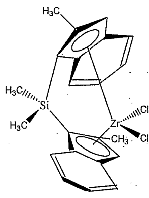
1,2-ethanediylbis(9-fluorenyl)zirconium dichloride,
