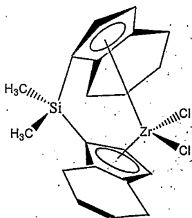
dimethylsilylbis(2-methyl-1-indenyl)zirconium dichloride,
