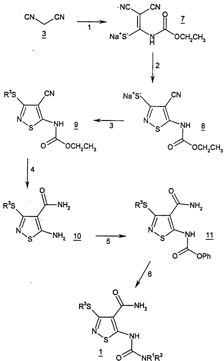
Scheme 2
