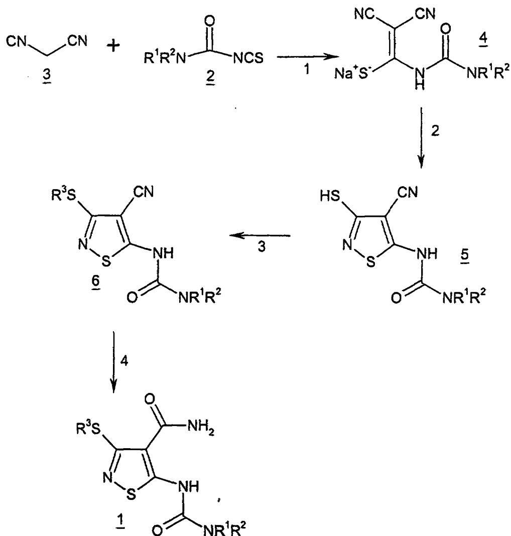
Scheme 1
