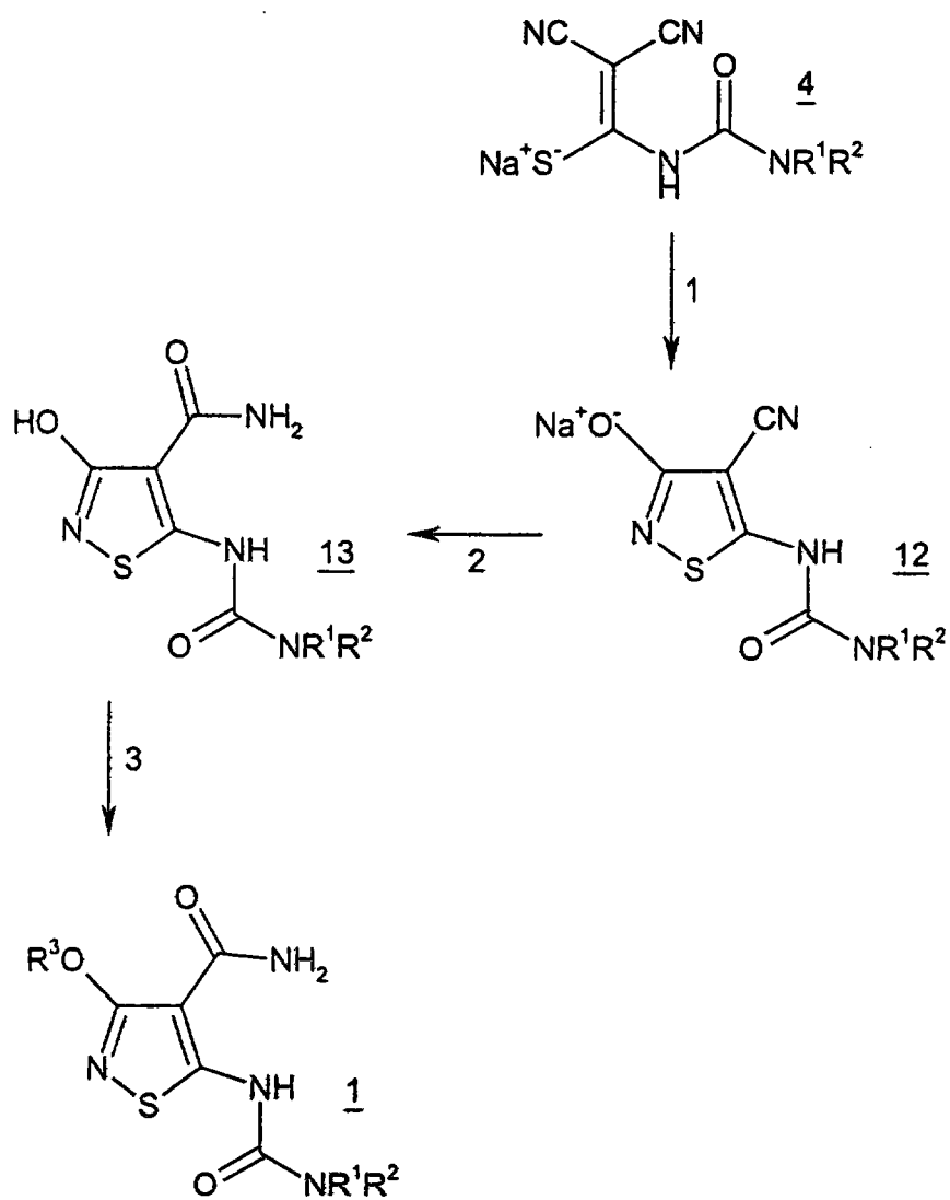
Scheme 3
