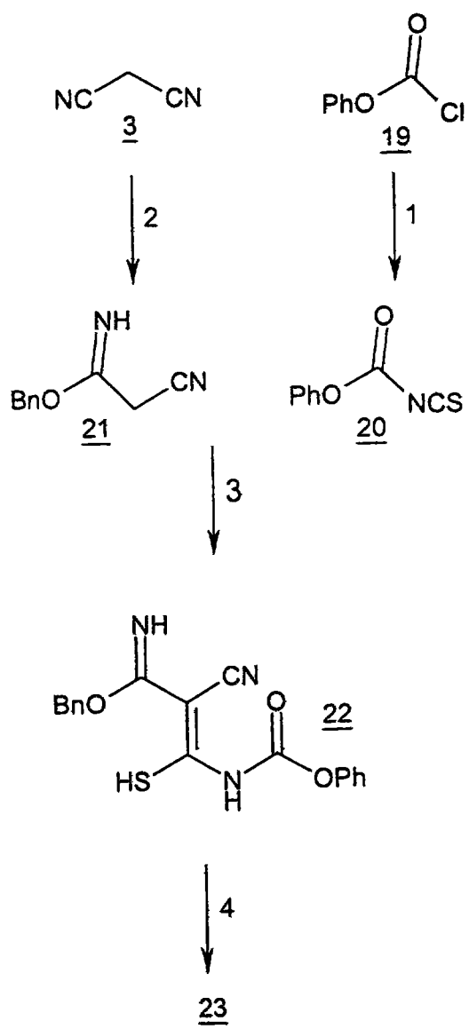
Scheme 5
