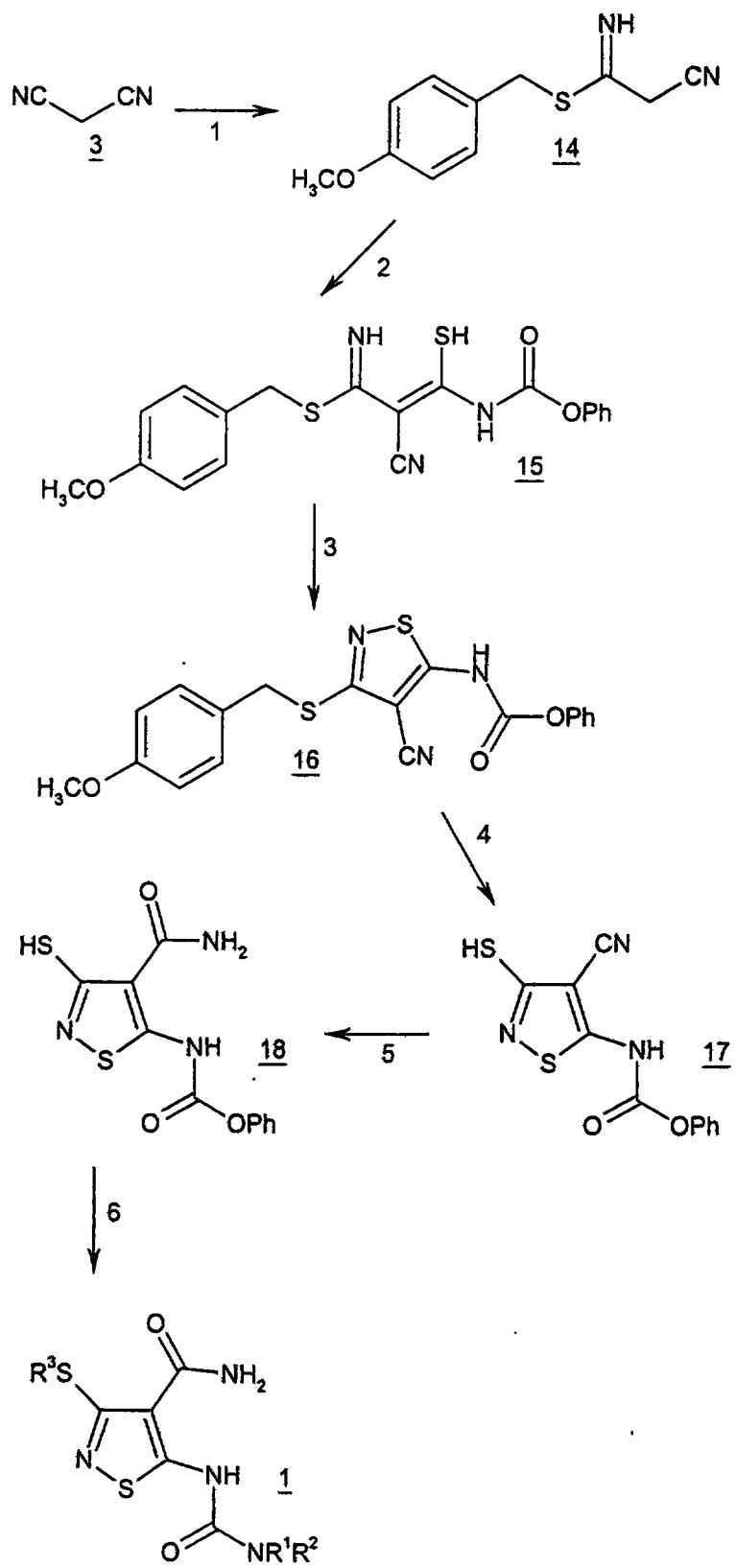
Scheme 4
