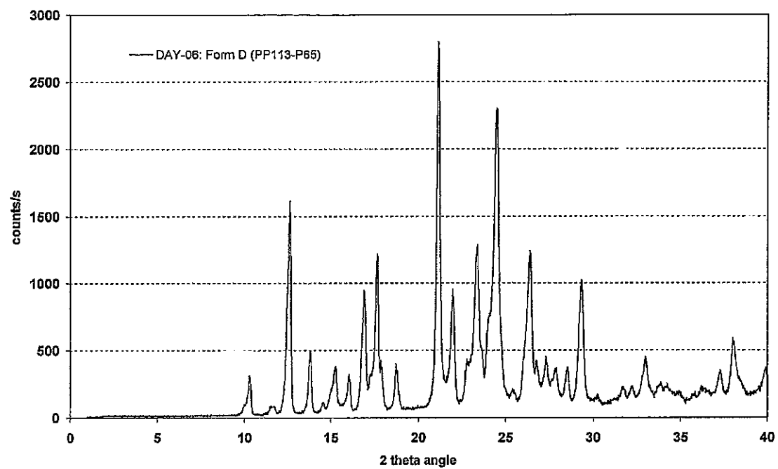
Figure 4 (N-desmethylozapine Form D)
