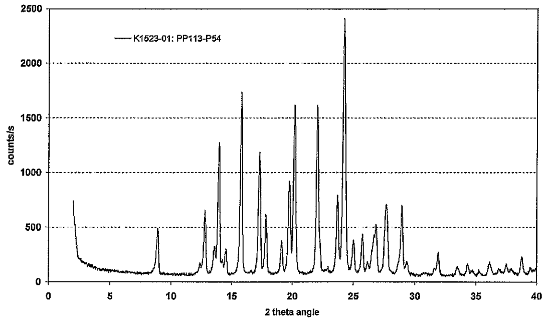
Figure 1 (N-desmethylozapine Form A)
