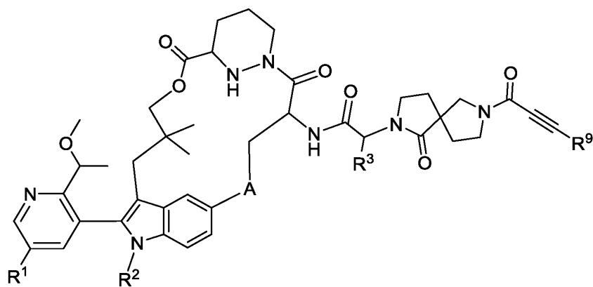
Formula II-6b.
