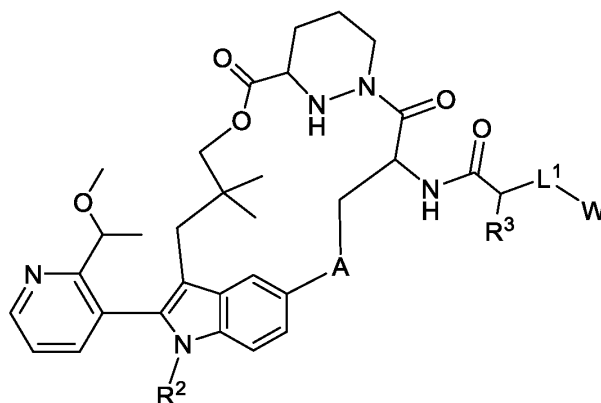
Formula II-1.
