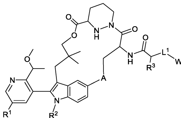
Formula I
