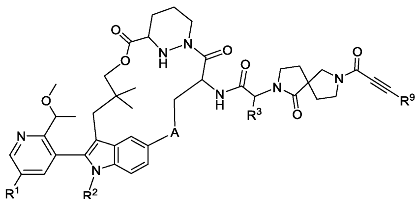
Formula II-6b.
