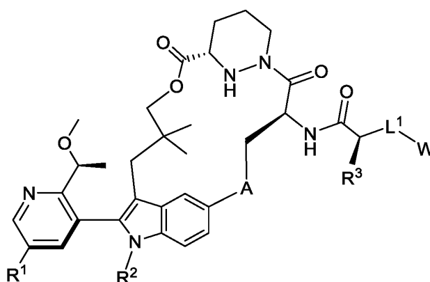
Formula Ia.
