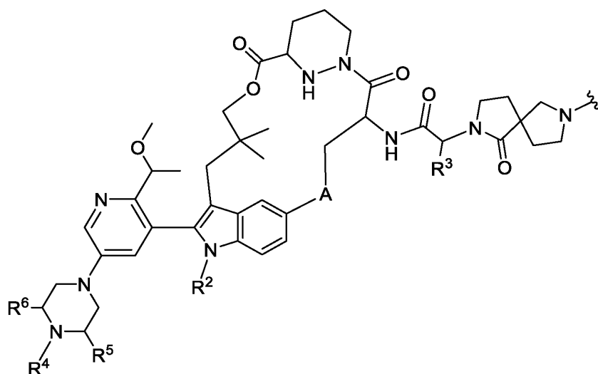
Formula VIc,
