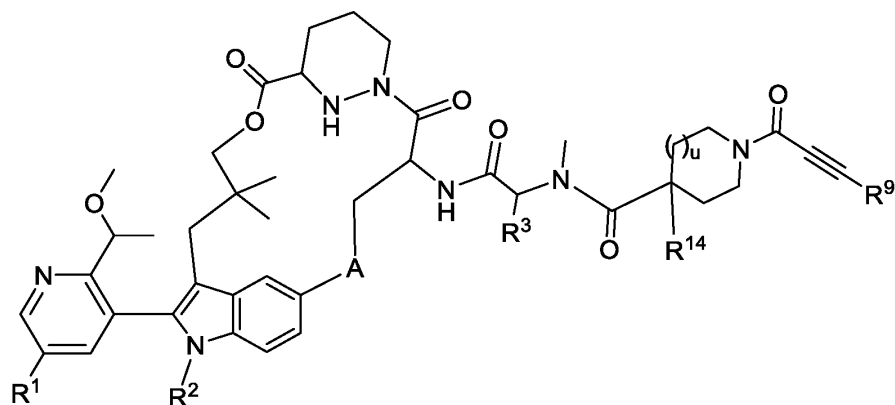
Formula II-6a,
