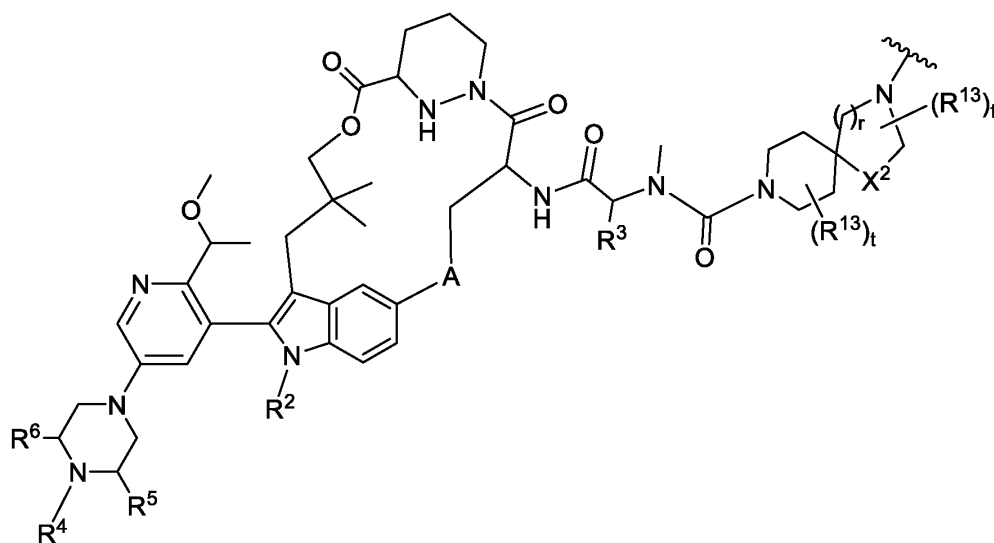
Formula VIa,
