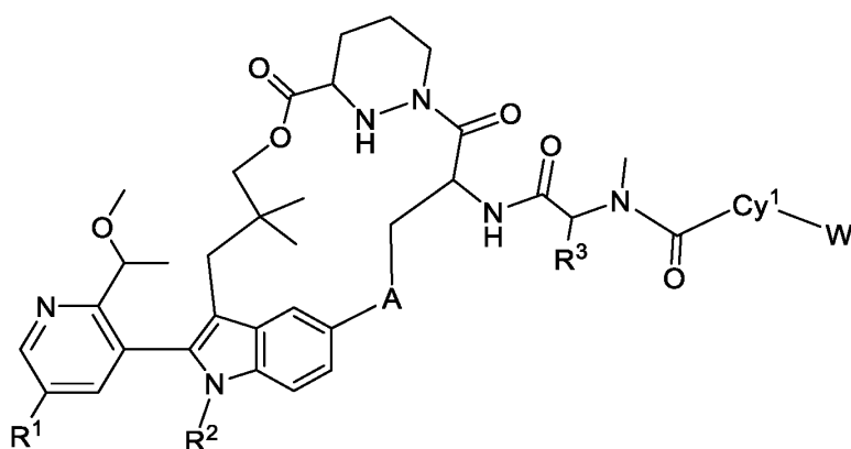
Formula II-5,
