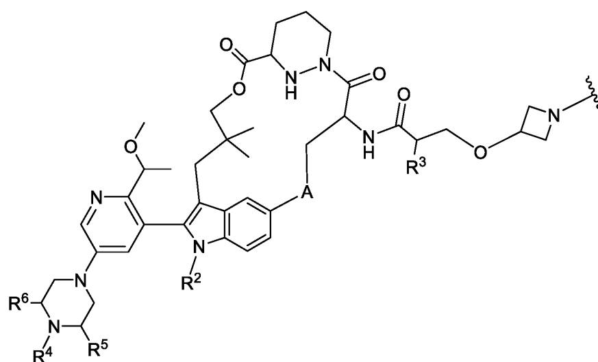
Formula VId,
