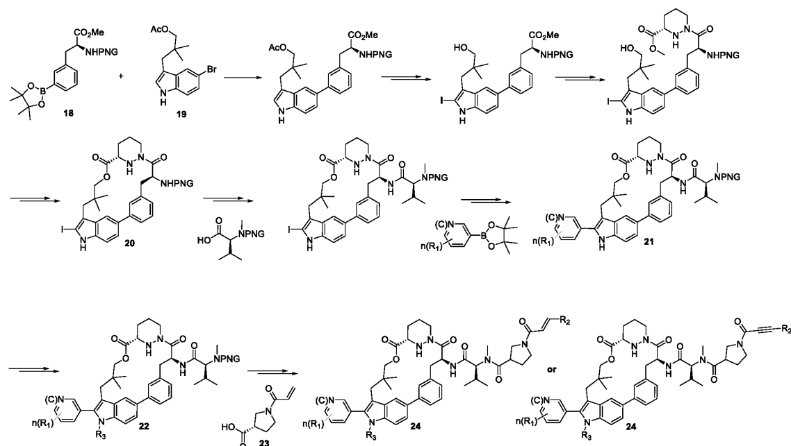
Scheme 5. General synthesis of macrocyclic esters
