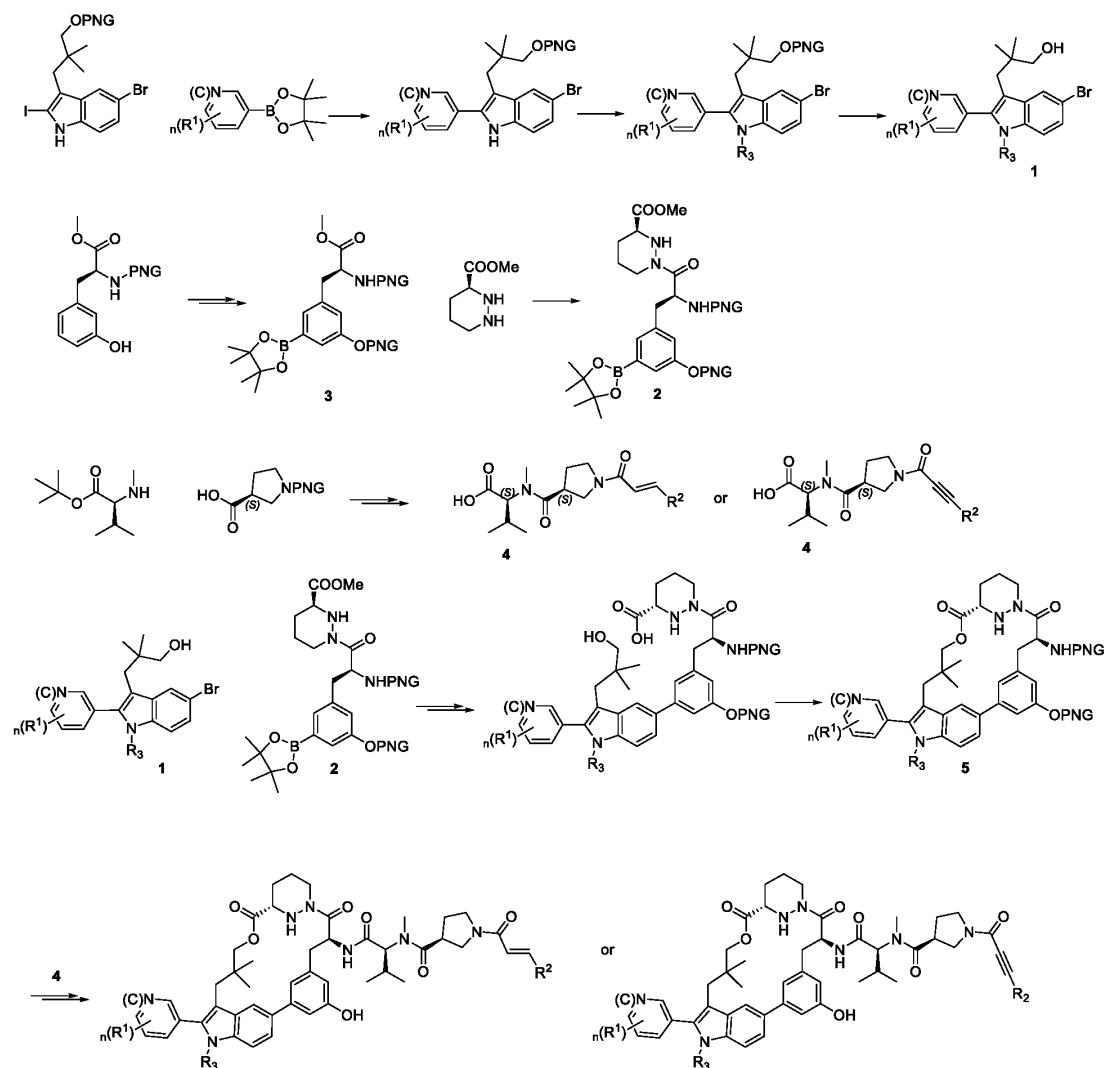
Scheme 1. General synthesis of macrocyclic esters
