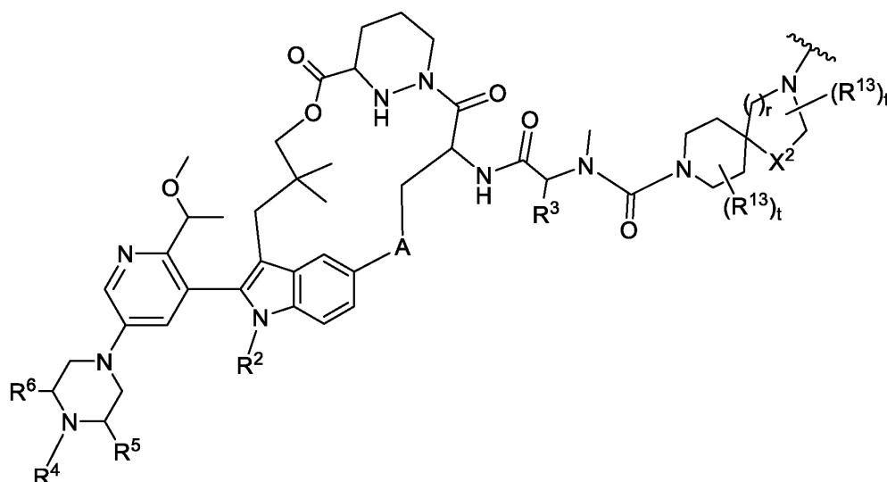
Formula VIa,
