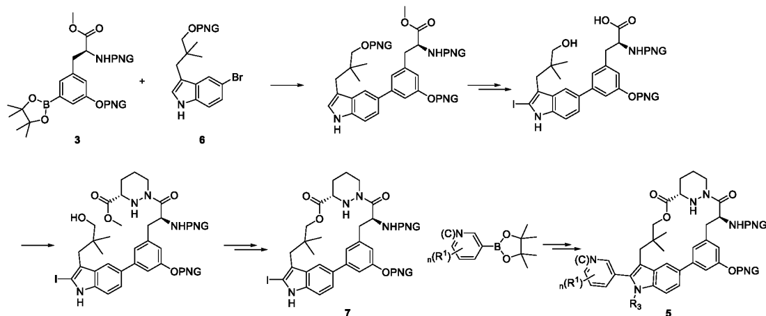
Scheme 2. Alternative general synthesis of macrocyclic esters
