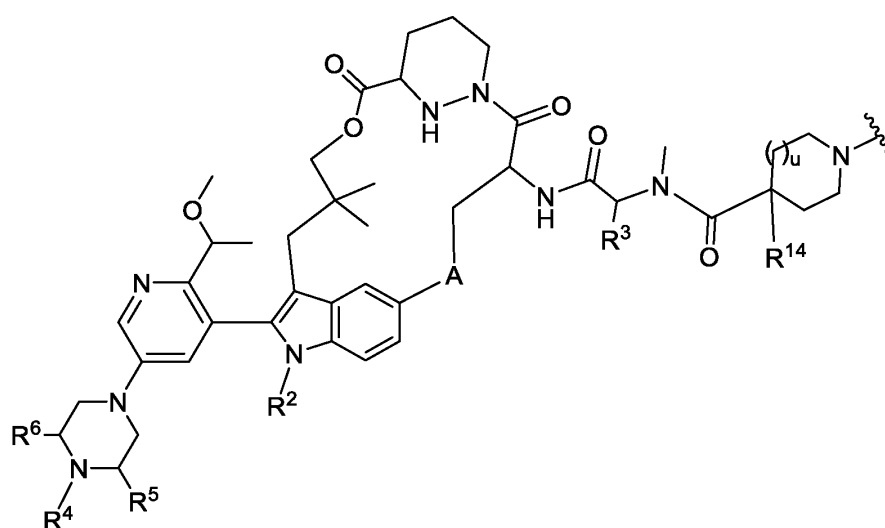
Formula VIb,
