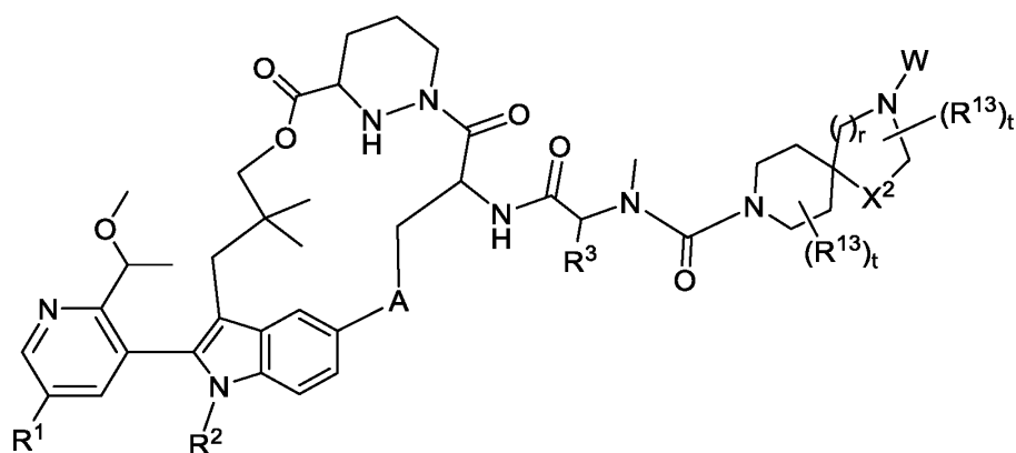
Formula II-5a,
