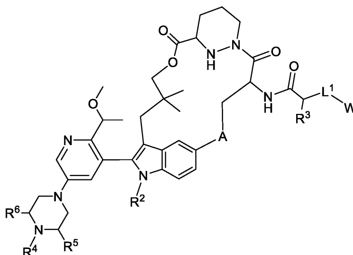
Formula II-2,
