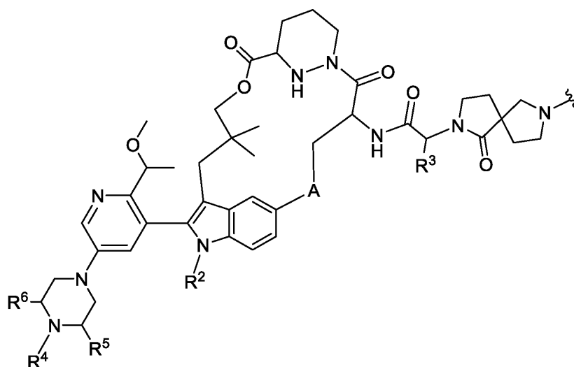
Formula VIc,
