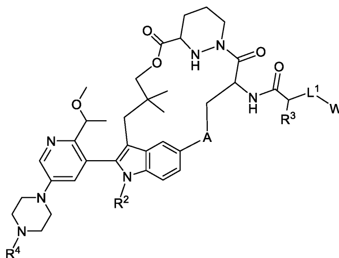
Formula II-3.
