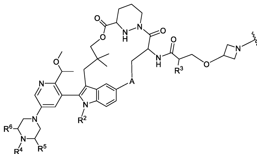
Formula VId,
