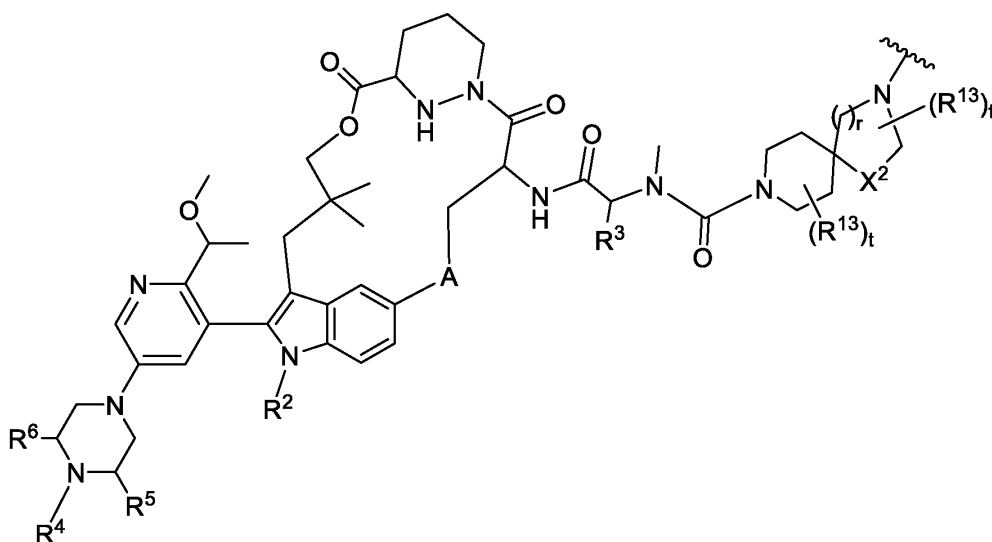
Formula VIa,
