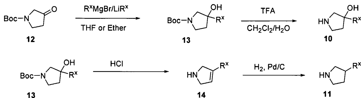
Scheme 4
