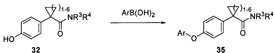
Scheme 12
