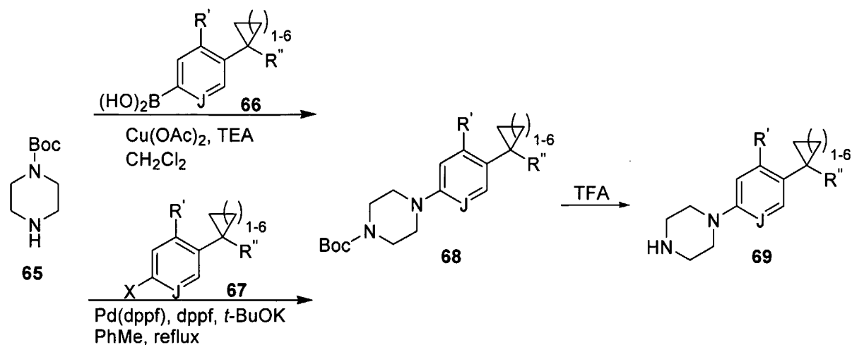
Scheme 17
