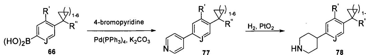
Scheme 20
