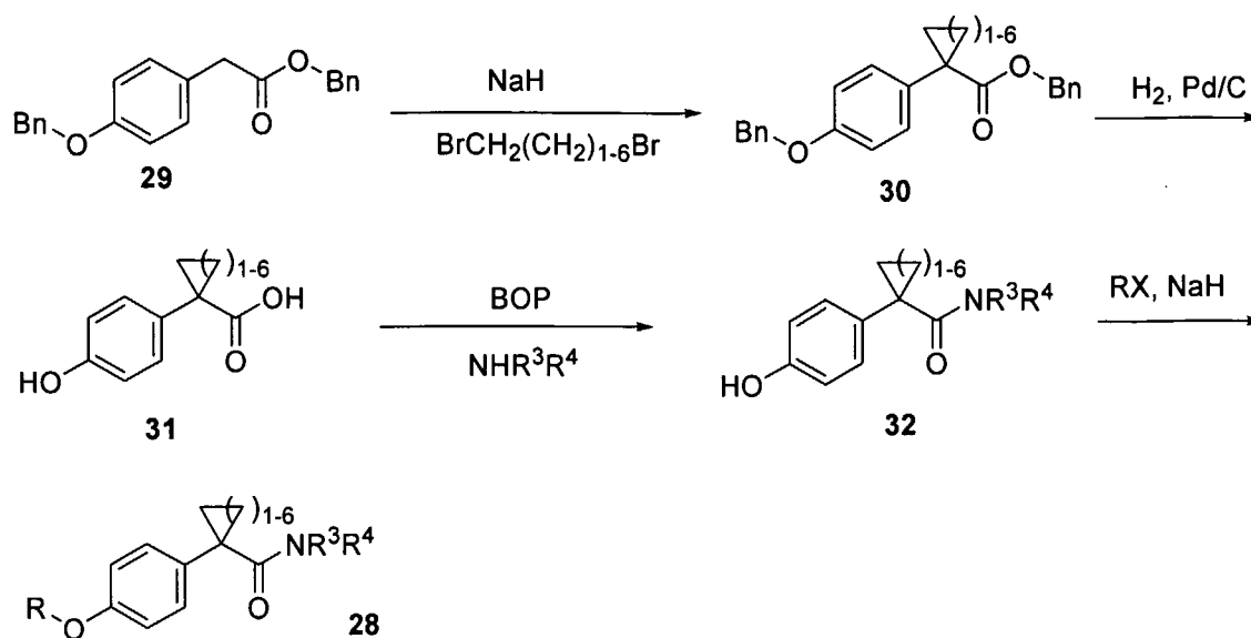
Scheme 10
