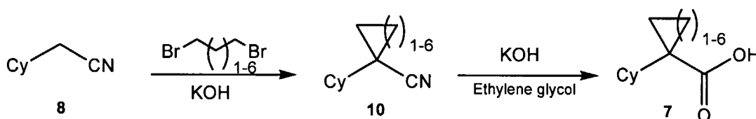
Scheme 3
