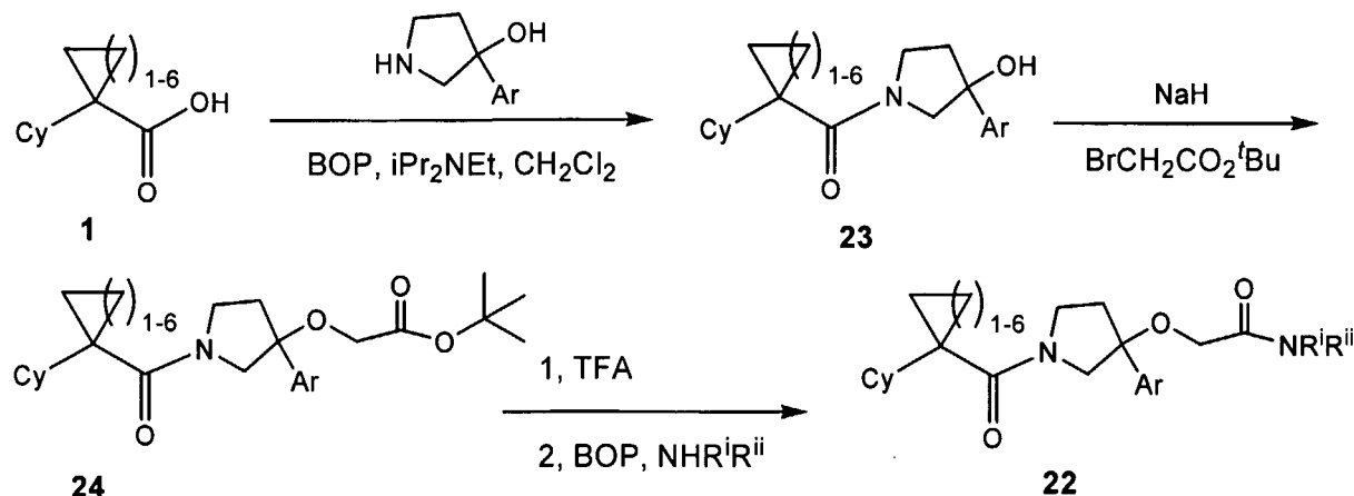
Scheme 8
