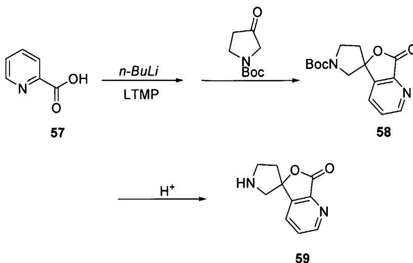
Scheme 15
