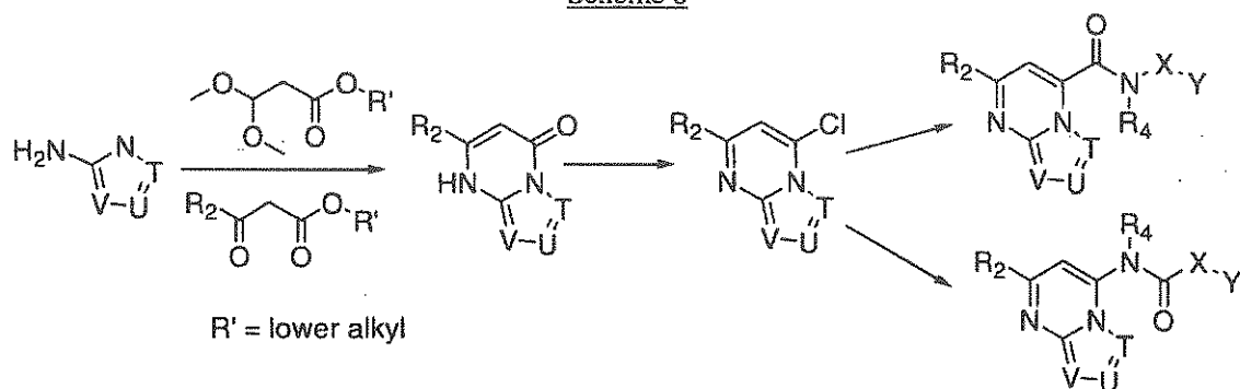
Scheme 8
