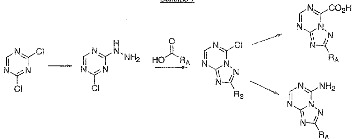
Scheme 7
