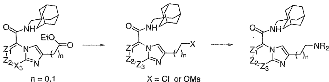
Scheme 13
