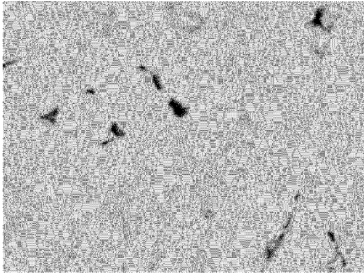
Ref.4:Sn-17In-2.5Ag-1.5Bi
