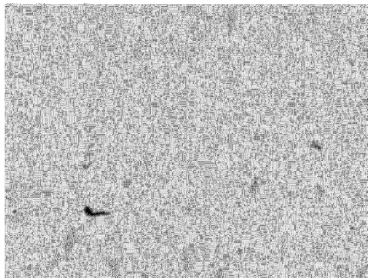
Ref.2:Sn-15.0In-2.5Ag-2.0Bi
