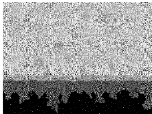
Ex.2:Sn-15.0In-2.5Ag-2.0Bi-0.02Ni
