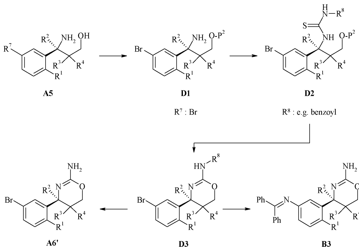
Scheme D: Alternative synthesis of intermediates A6' and B3 .
