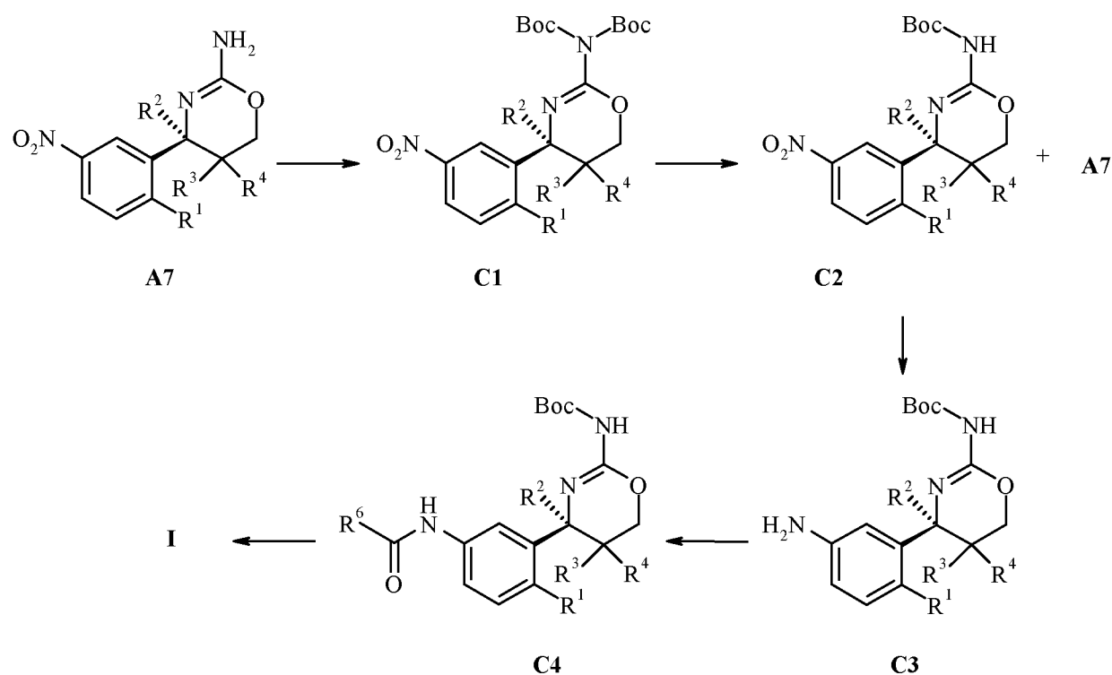
Scheme C: Alternative synthesis of compounds of formula I .
