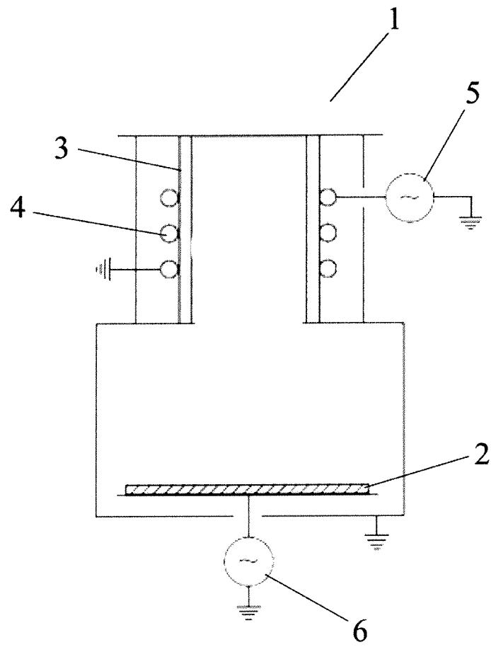
Fig. 1 (Prior Art)
