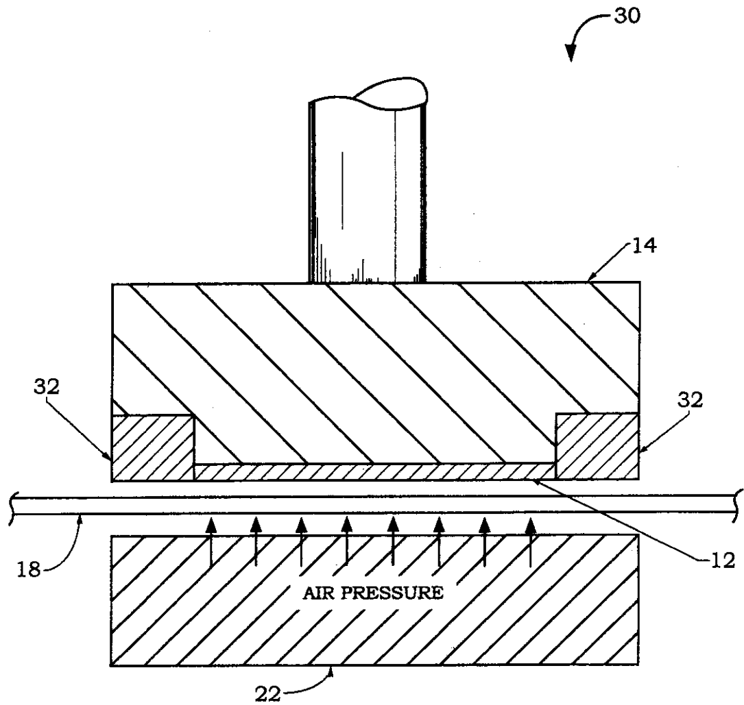
FIG. 2 (Prior Art)
