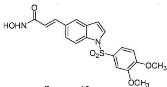
Compound 8
