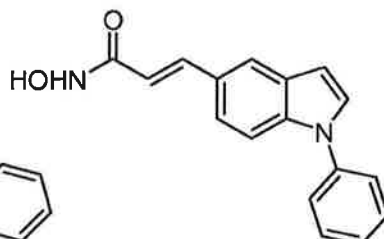
Compound 11
