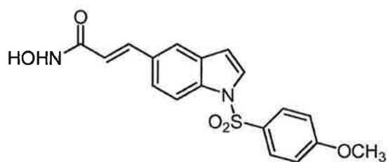
Compound 4
