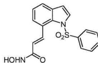
Compound 19
