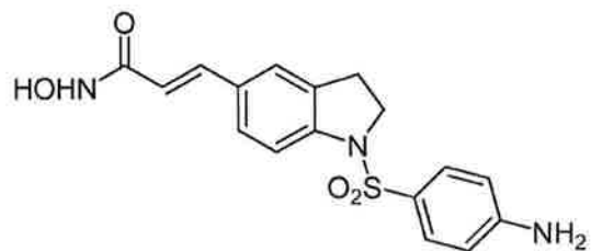
Compound 16
