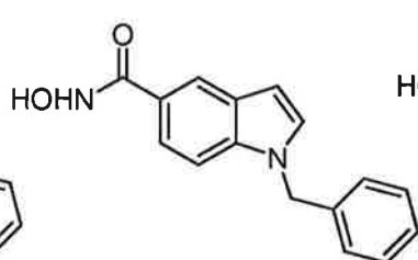
Compound 2
