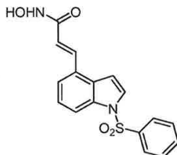
Compound 21
