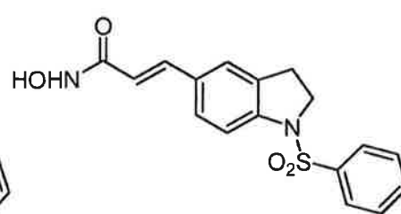
Compound 12
