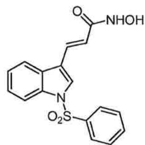
Compound 19
