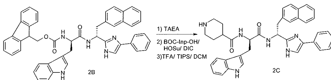
Scheme 2C
