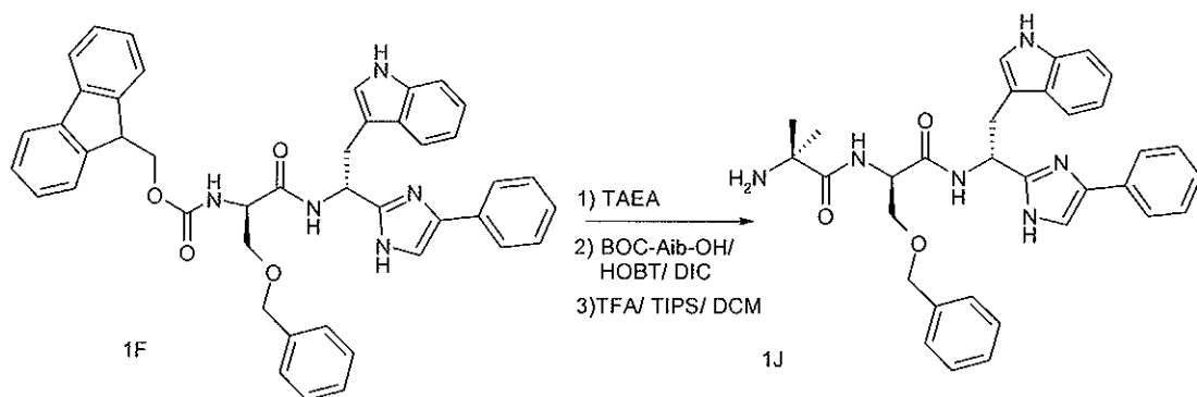
Scheme 1J
