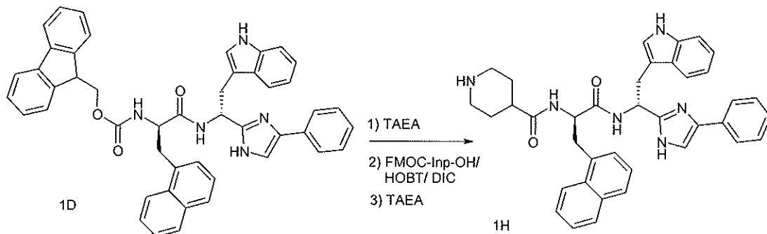
Scheme 1I
