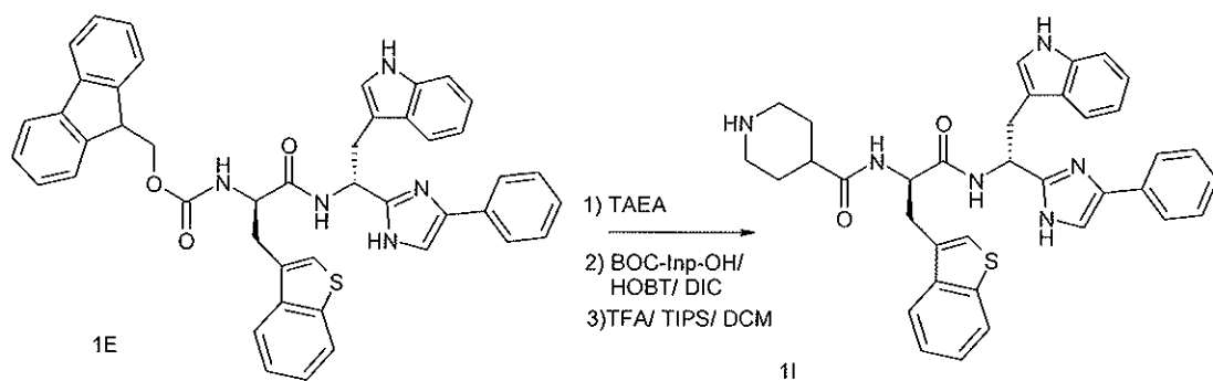
Scheme 1J
