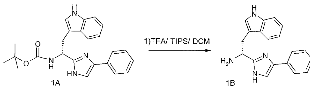
Scheme 1B
