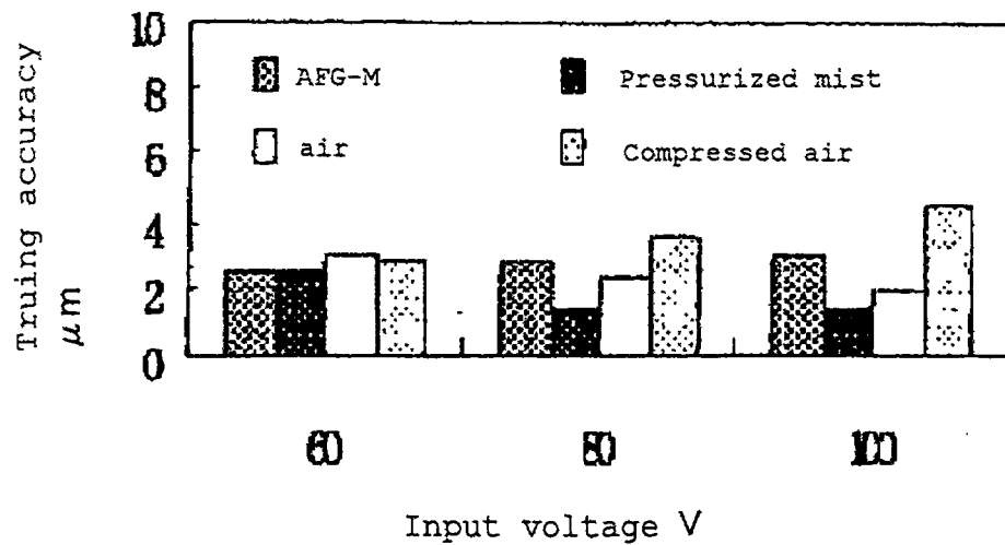
Accuracies (roundness) of grindstone after truing
