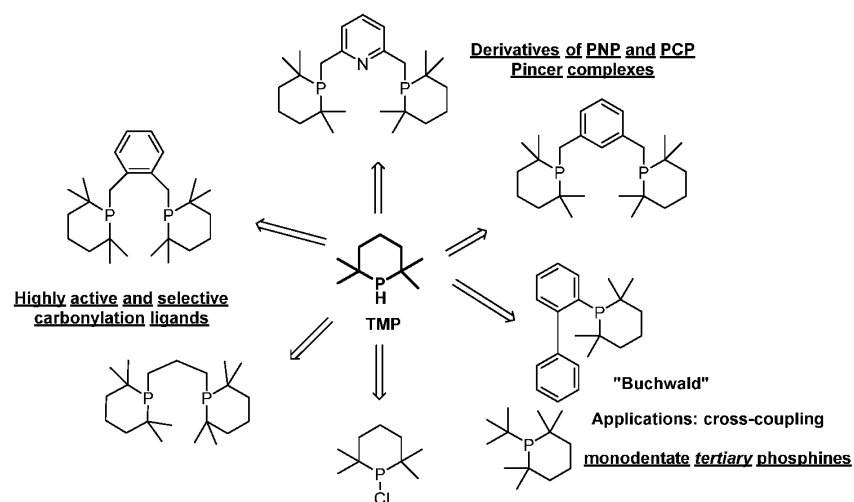
Scheme 1. Compound derivatives of the present invention
