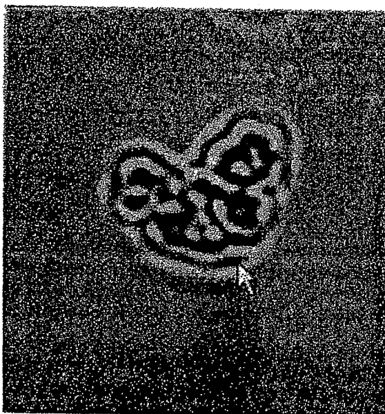
Breakage of oocyst after contact with active surface.
