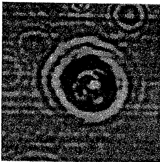
Cryptosporidium oocyst adsorbed on sand remains unaffected.
