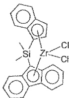
(complex 16)
