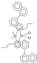
(complex 11)
