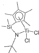
(complex 4)
