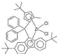
(complex 7)
