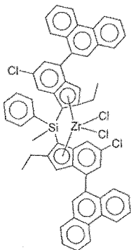
(complex 12)
