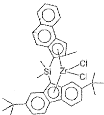
(Complex 1)
