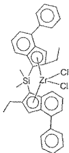
(complex 9)
