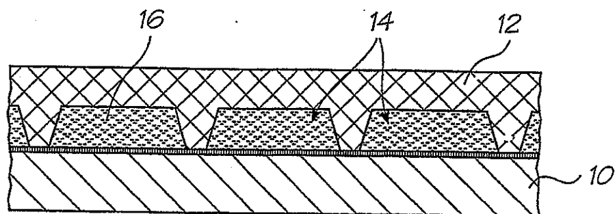
FIG. 1 (Prior Art)
