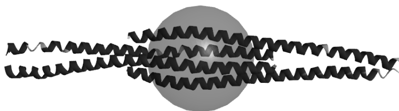
Vimentin (3KLT)
