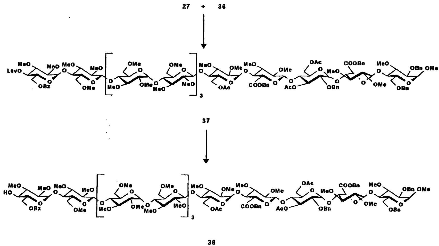
SCHEME 8 - Synthesis of the polysaccharide 38
