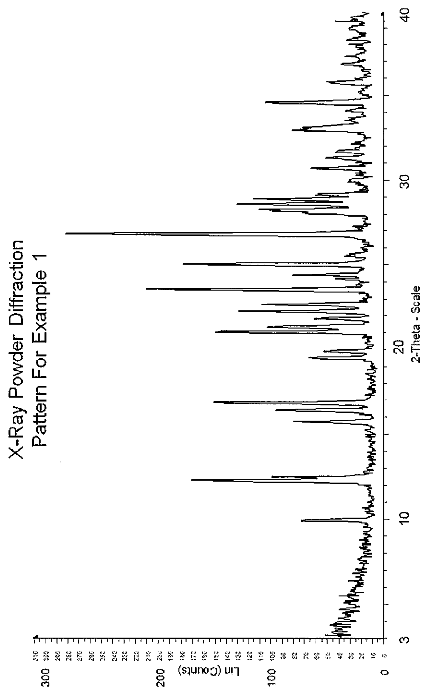
FIG. 1. X-ray powder diffraction pattern for Example 1.
