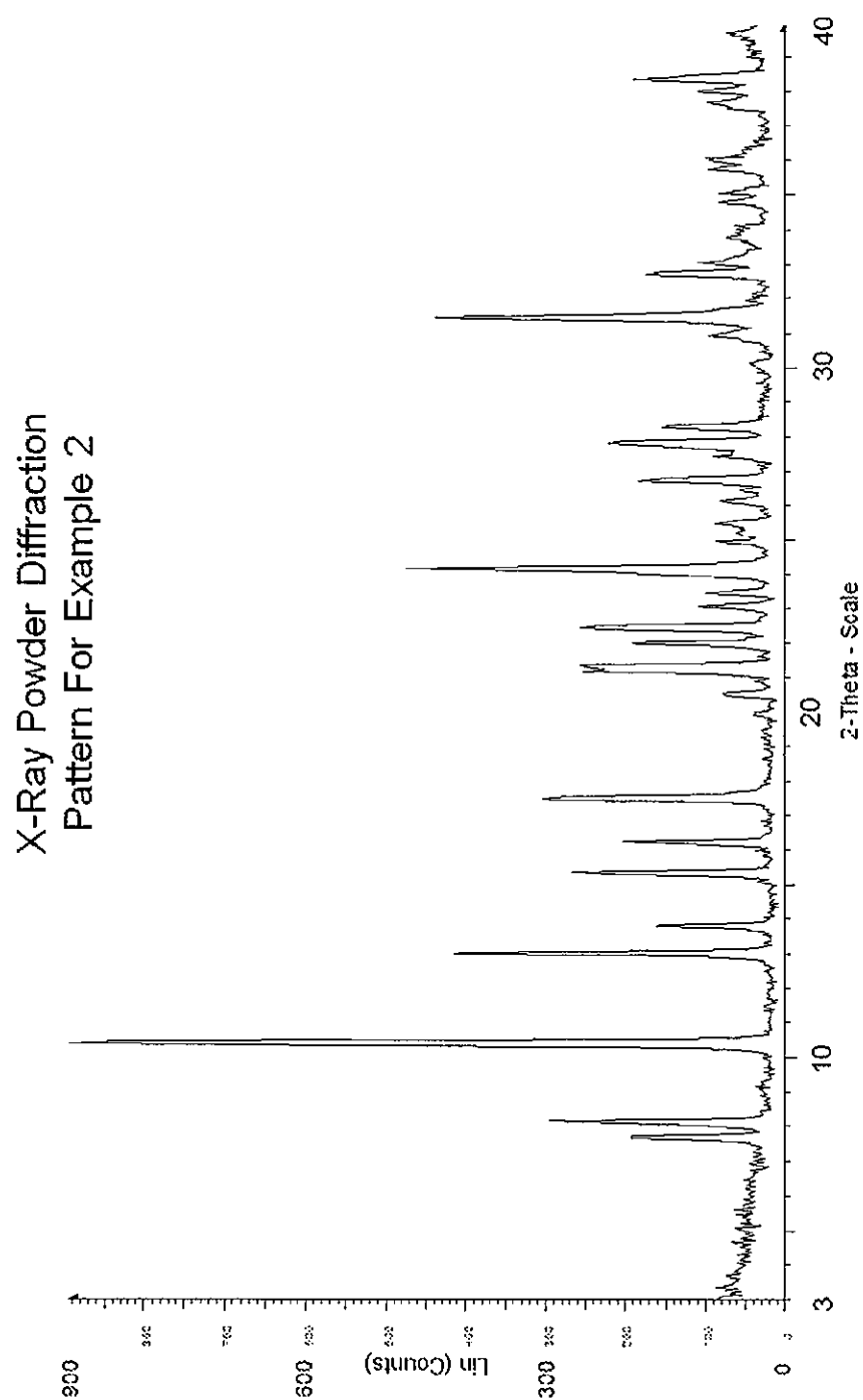
FIG. 2. X-ray powder diffraction pattern of Example 2.
