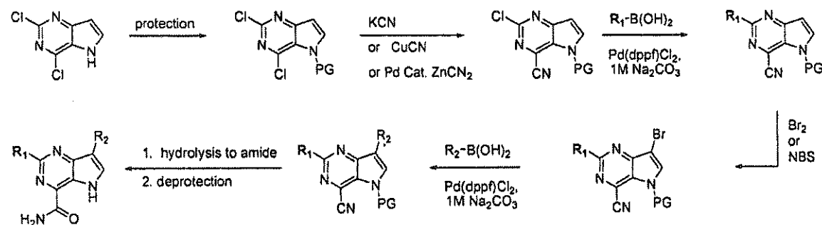
[00165] Scheme 7:
