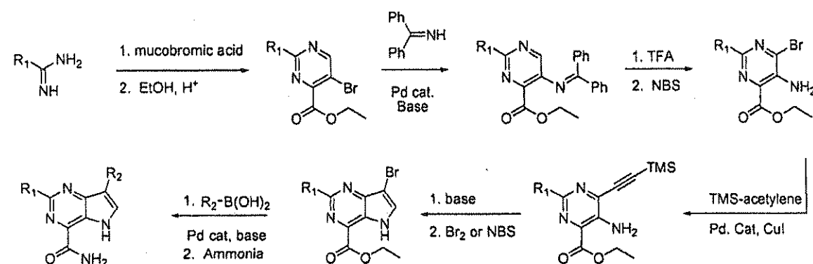
[00166] Scheme 8:
