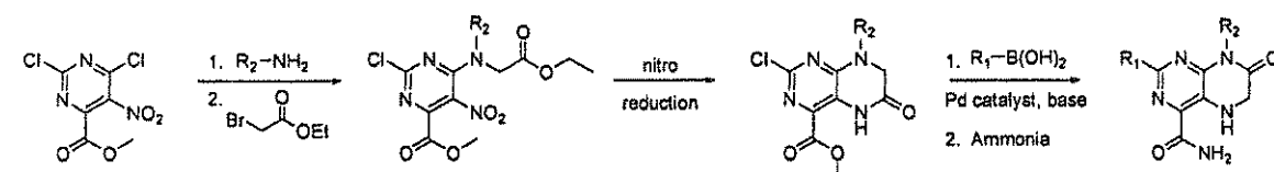
[00166] Scheme 8:
