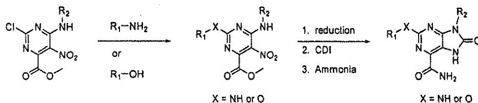
[00163] Scheme 5:
