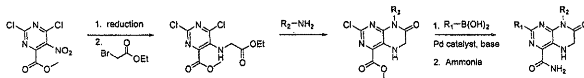
[00163] Scheme 5:
