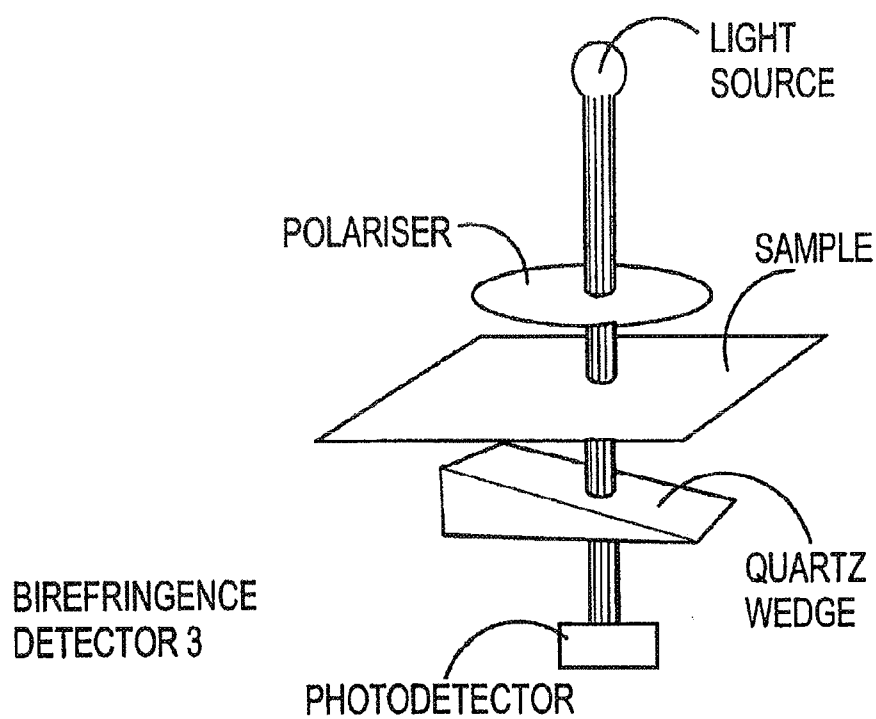
FIG. 3 (PRIOR ART)
