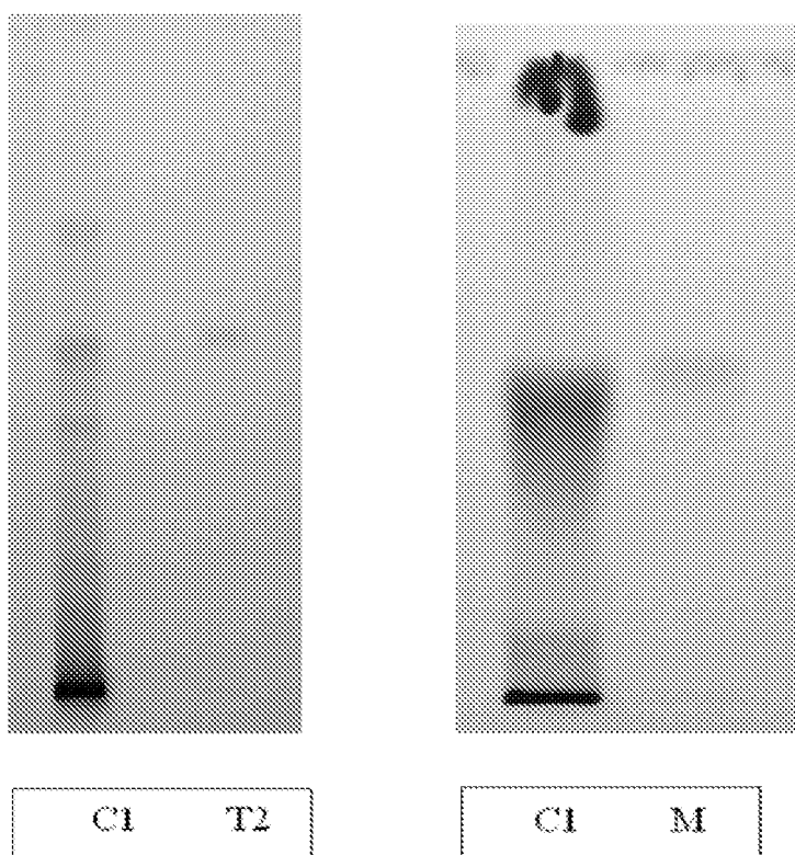
Figure 1: HPTLC Fingerprint images of Salacia composition
