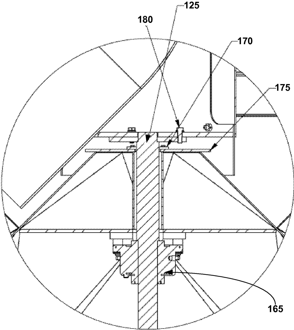
DETAIL B
