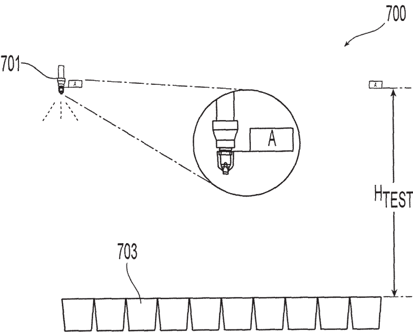
Elevation View
