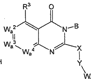
Formula VIII
