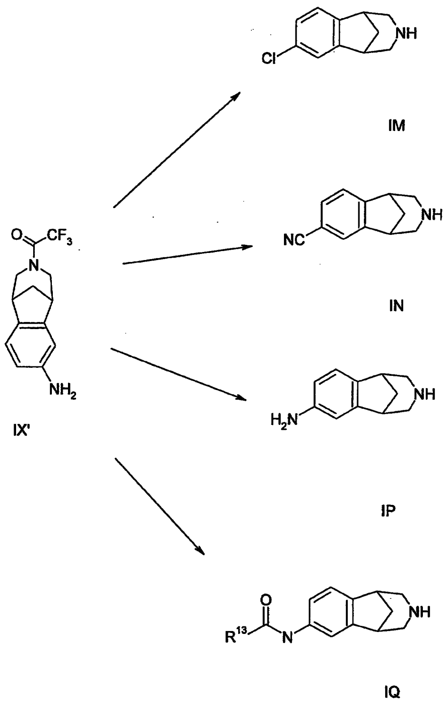
Scheme 10
