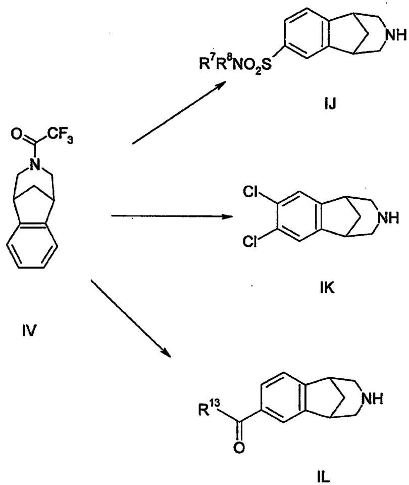
Scheme 9
