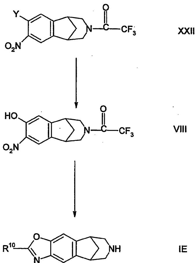
Scheme 5
