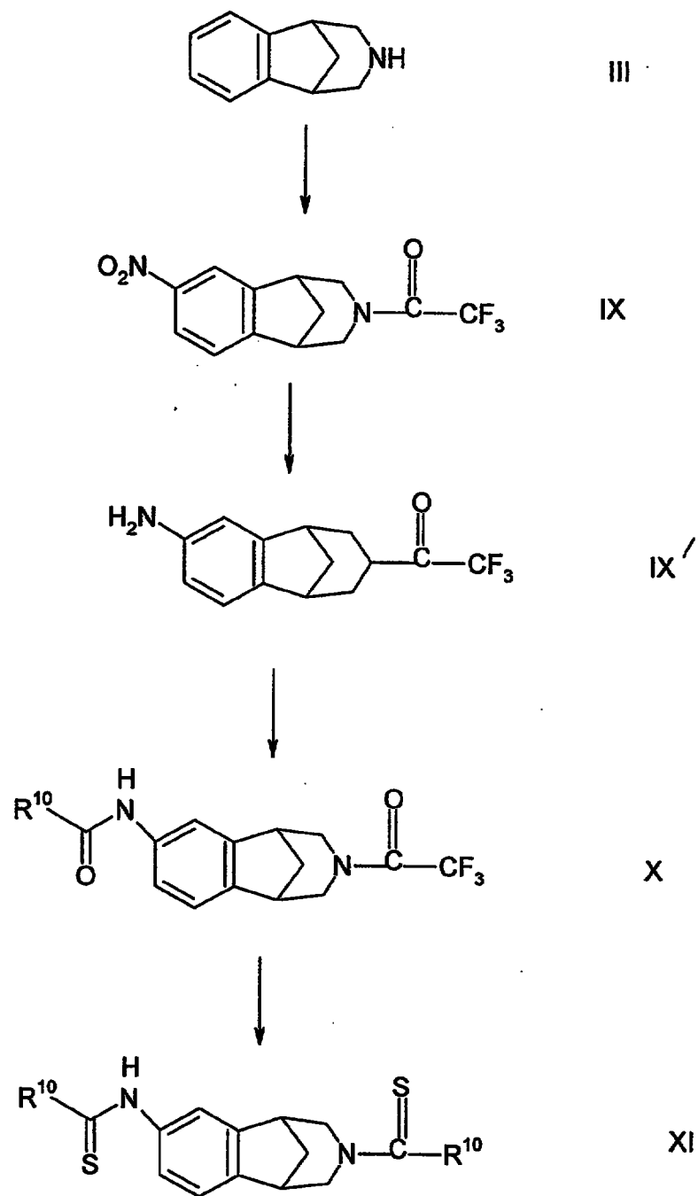
Scheme 6
