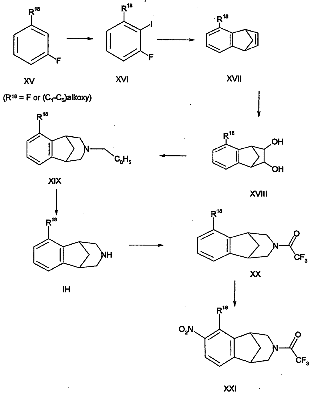
Scheme 8
