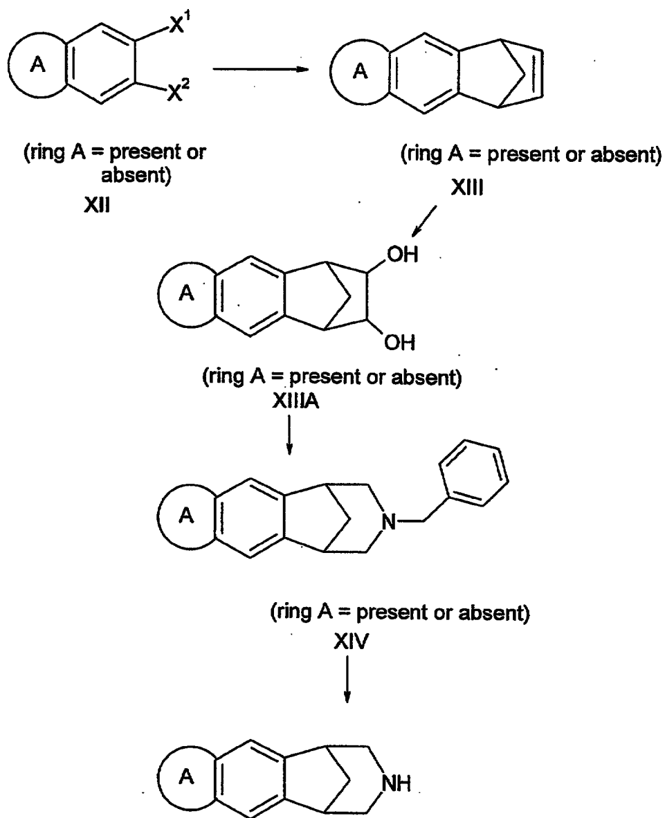
Scheme 7
