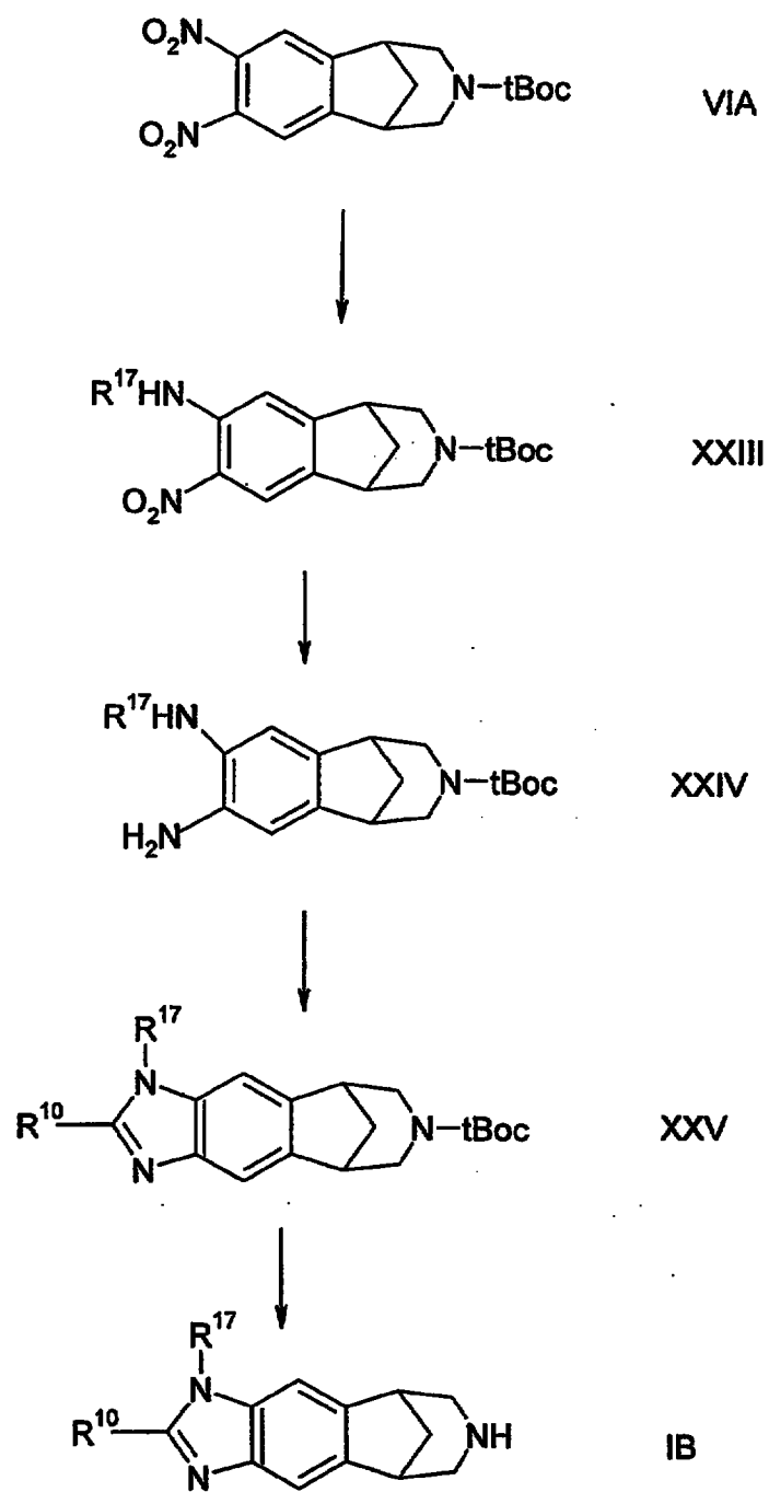
Scheme 3
