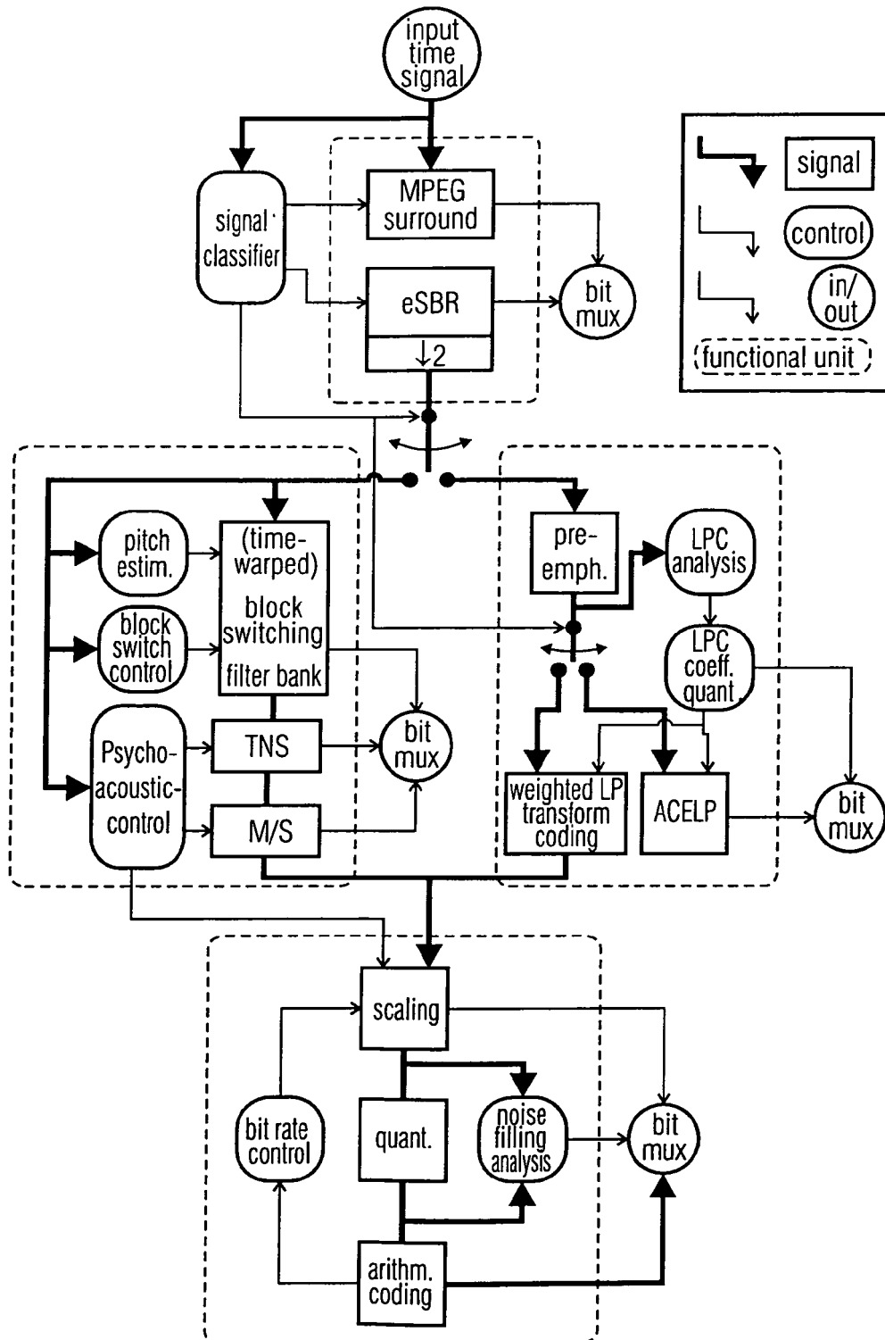
Block Diagram of the USAC encoder FIG 5A (PRIOR ART)
