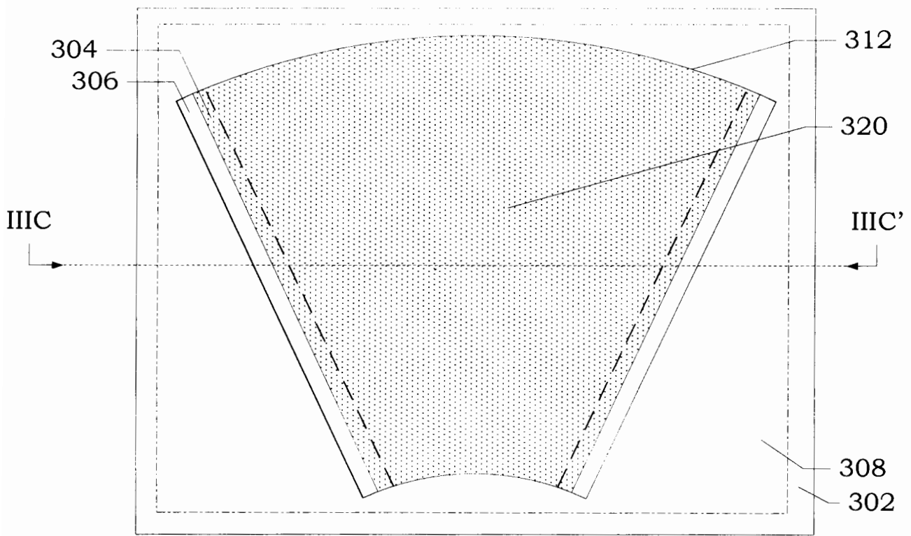
FIG. 3D (top view)
