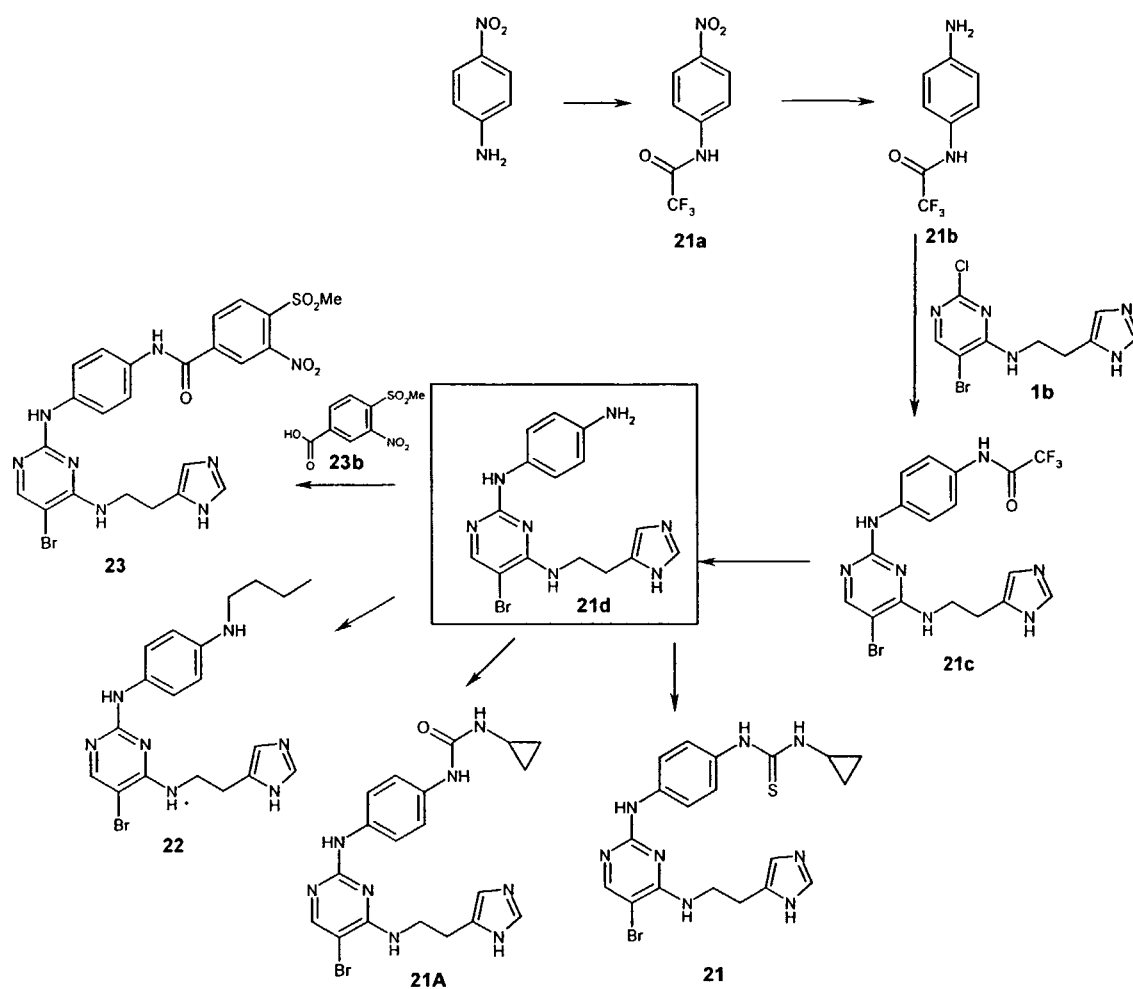
Scheme 21
